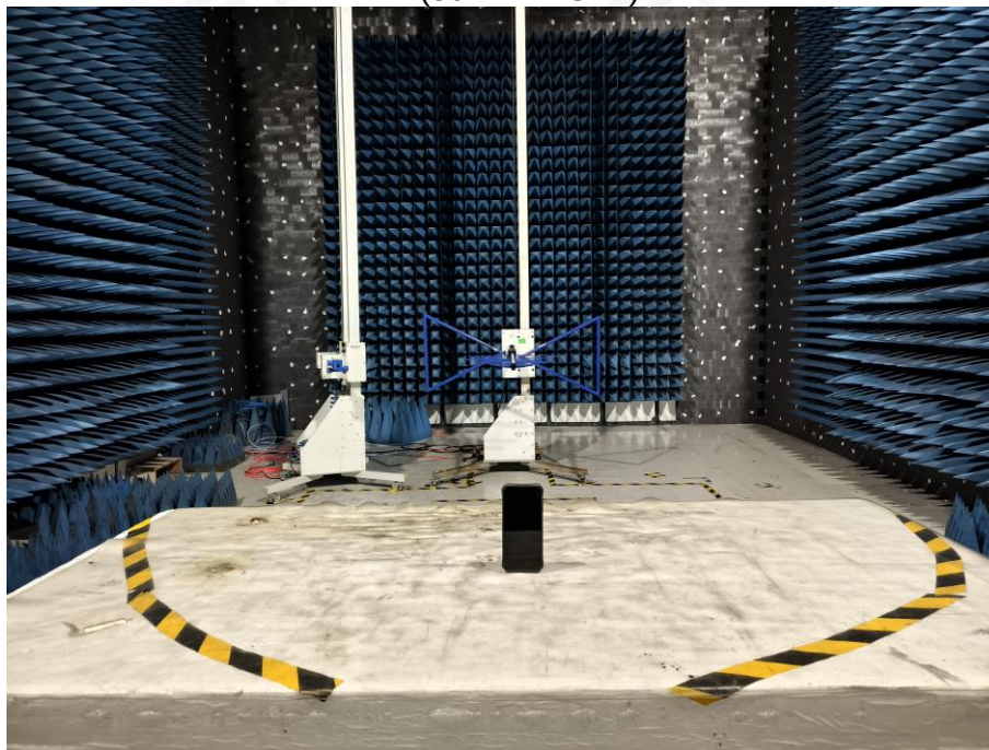
RE (30 MHz-1GHz)
