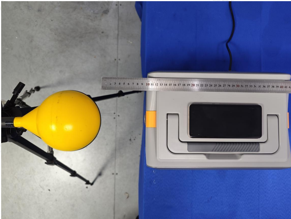
Test Position C(10cm) - Exposure photo from side edge surface-Left(TM4)
