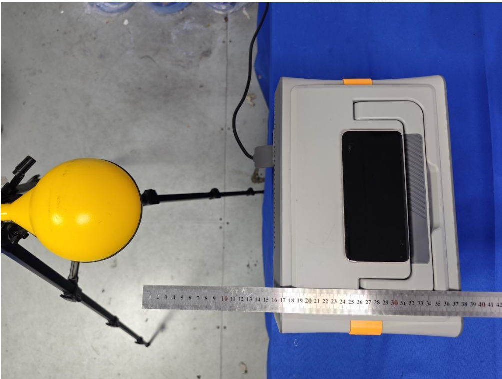
Test Position D(16cm) - Exposure photo from side edge surface-Front(TM4)
