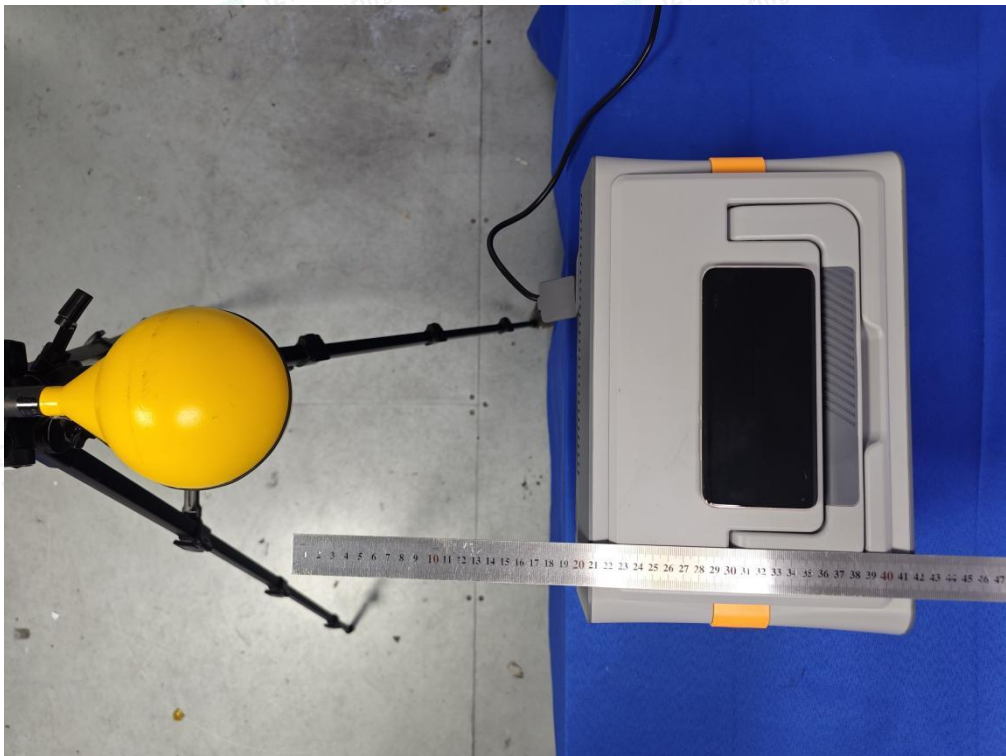
Test Position D(20cm) - Exposure photo from side edge surface-Front(TM4)
