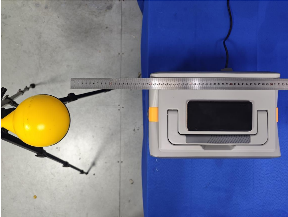
Test Position C(20cm) - Exposure photo from side edge surface-Left(TM4)
