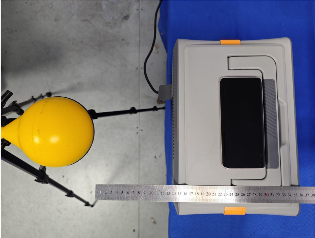
Test Position D(14cm) - Exposure photo from side edge surface-Front(TM4)
