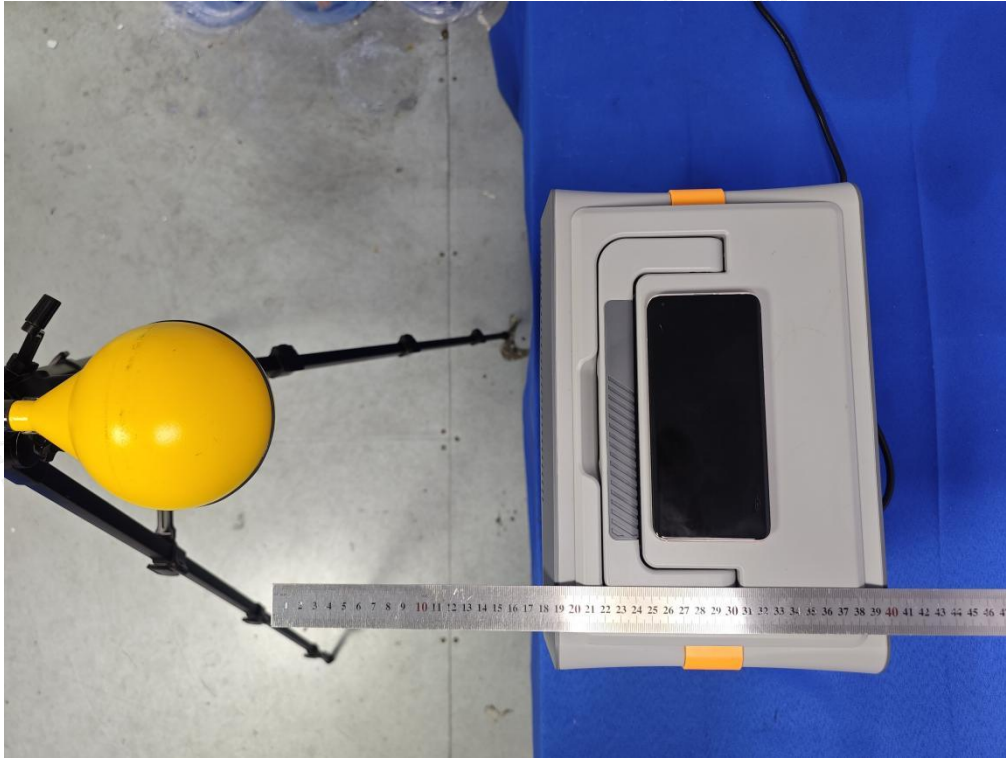
Test Position B(18cm) - Exposure photo from side edge surface-Rear(TM4)
