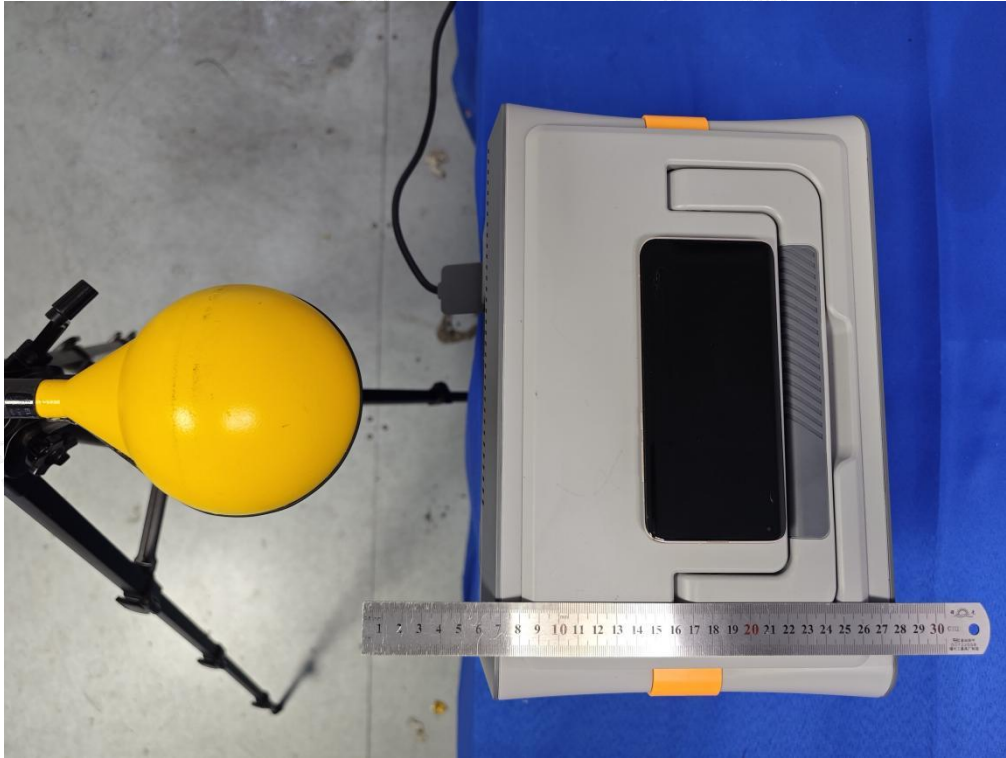
Test Position D(6cm) - Exposure photo from side edge surface-Front(TM4)
