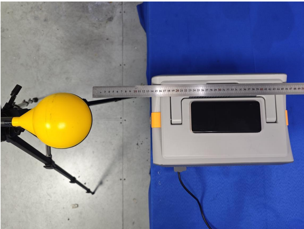
Test Position E(14cm) - Exposure photo from side edge surface-Right(TM4)
