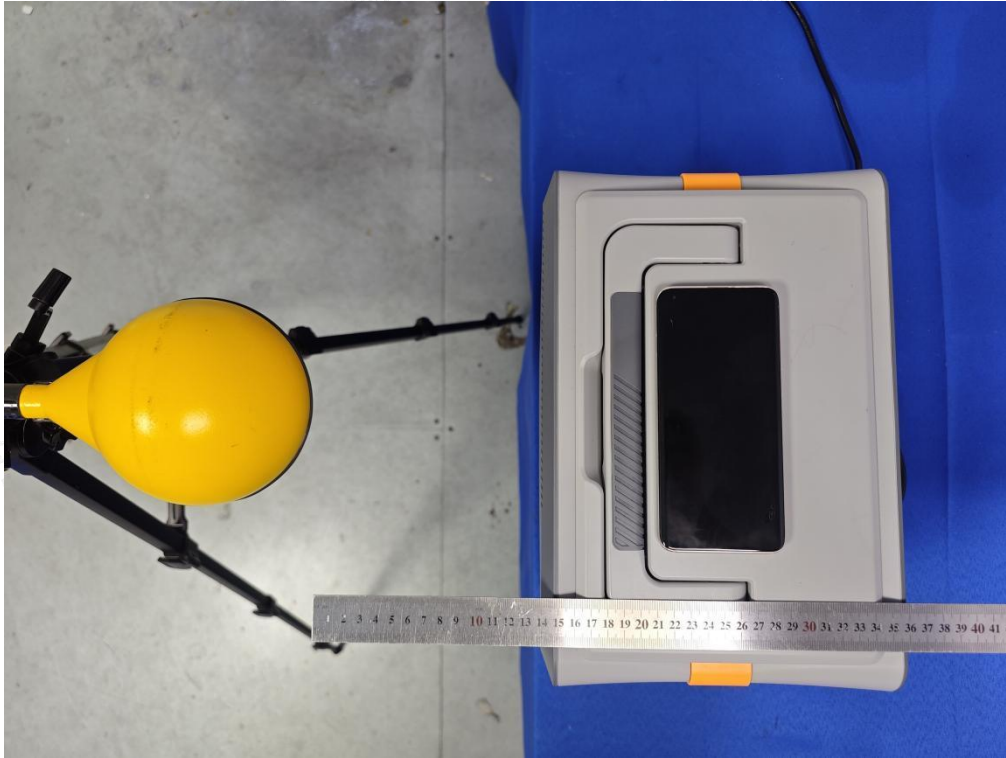
Test Position B(14cm) - Exposure photo from side edge surface-Rear(TM4)
