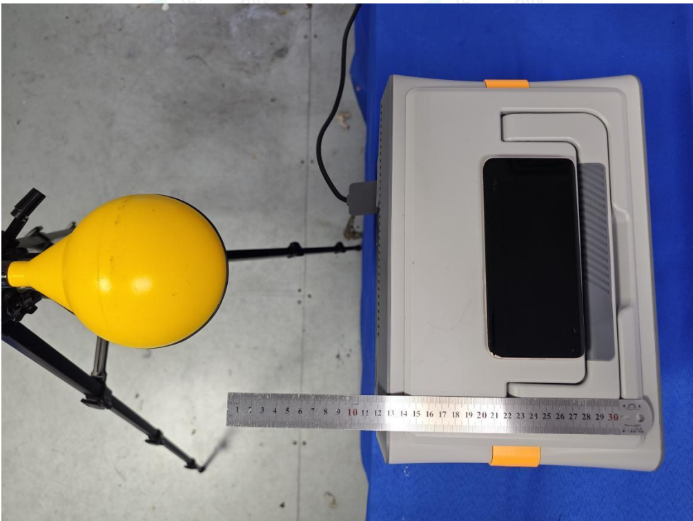
Test Position D(12cm) - Exposure photo from side edge surface-Front(TM4)
