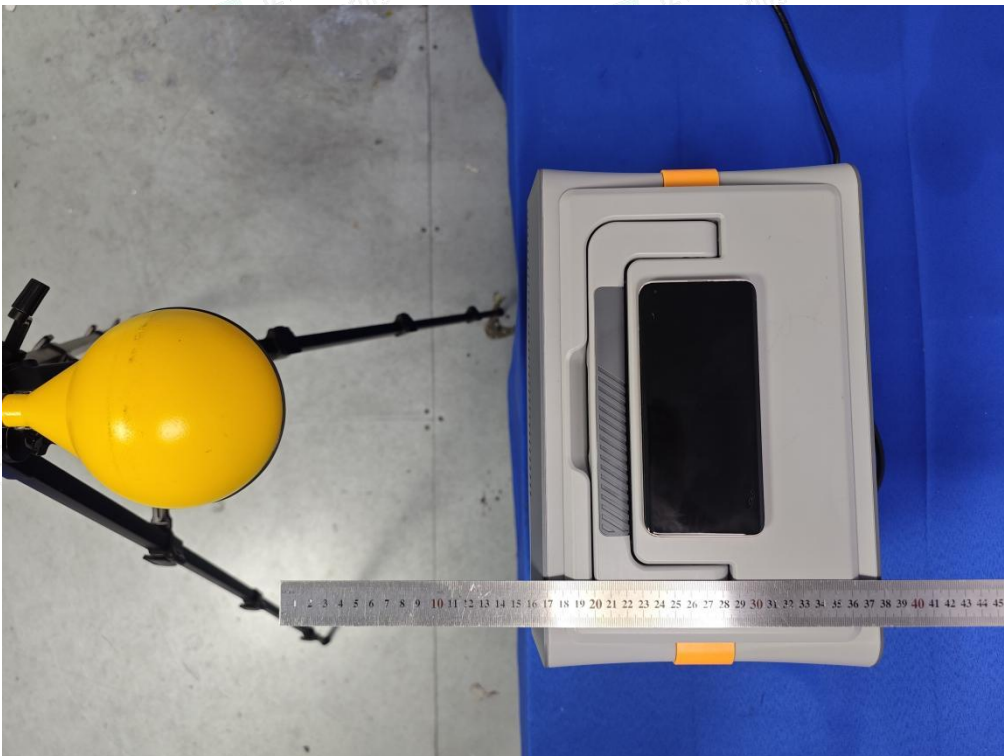
Test Position B(16cm) - Exposure photo from side edge surface-Rear(TM4)
