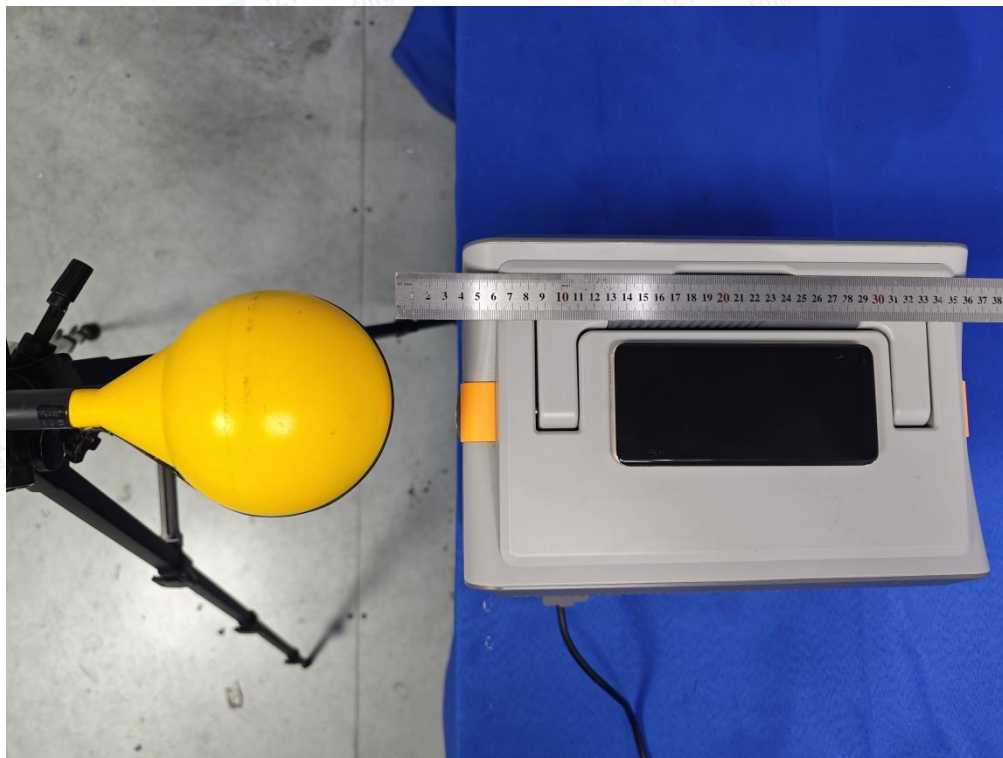
Test Position E(4cm) - Exposure photo from side edge surface-Right(TM4)
