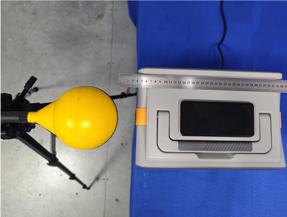
Test Position C(4cm) - Exposure photo from side edge surface-Left(TM4)
