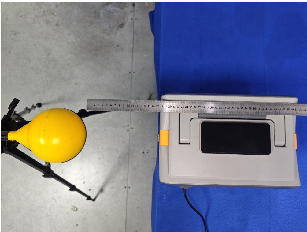
Test Position E(18cm) - Exposure photo from side edge surface-Right(TM4)
