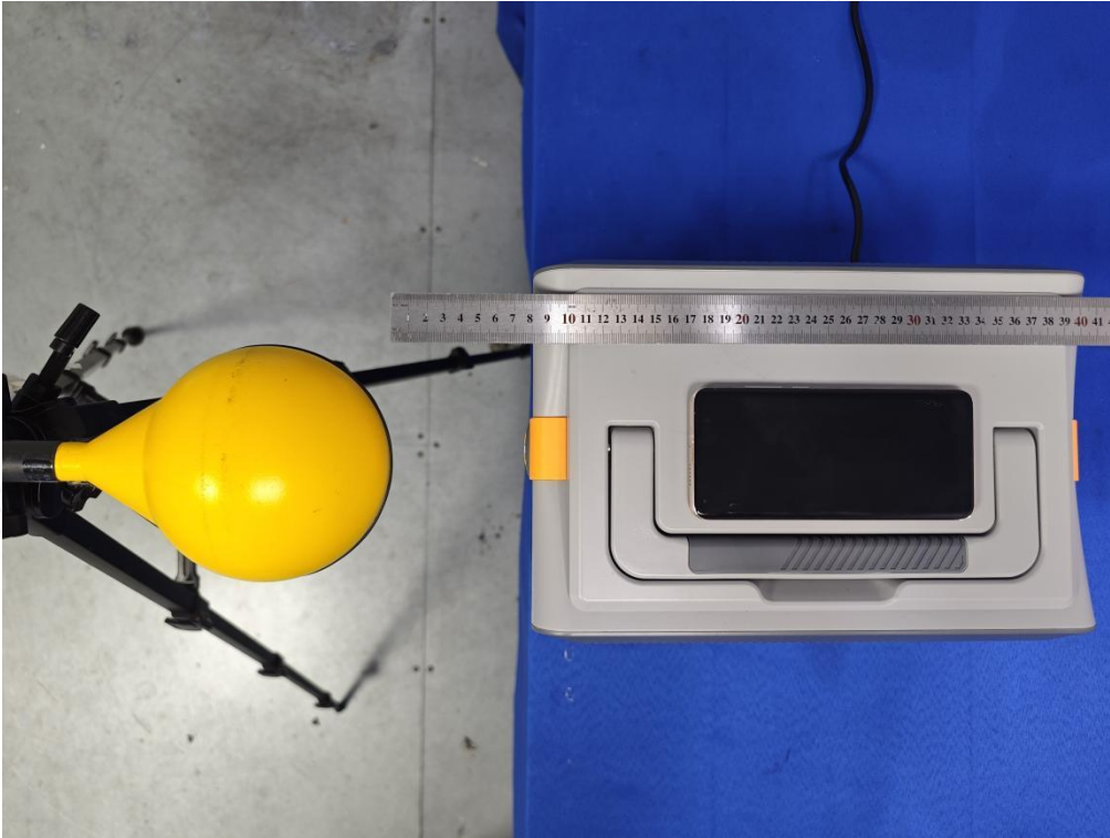
Test Position C(8cm) - Exposure photo from side edge surface-Left(TM4)
