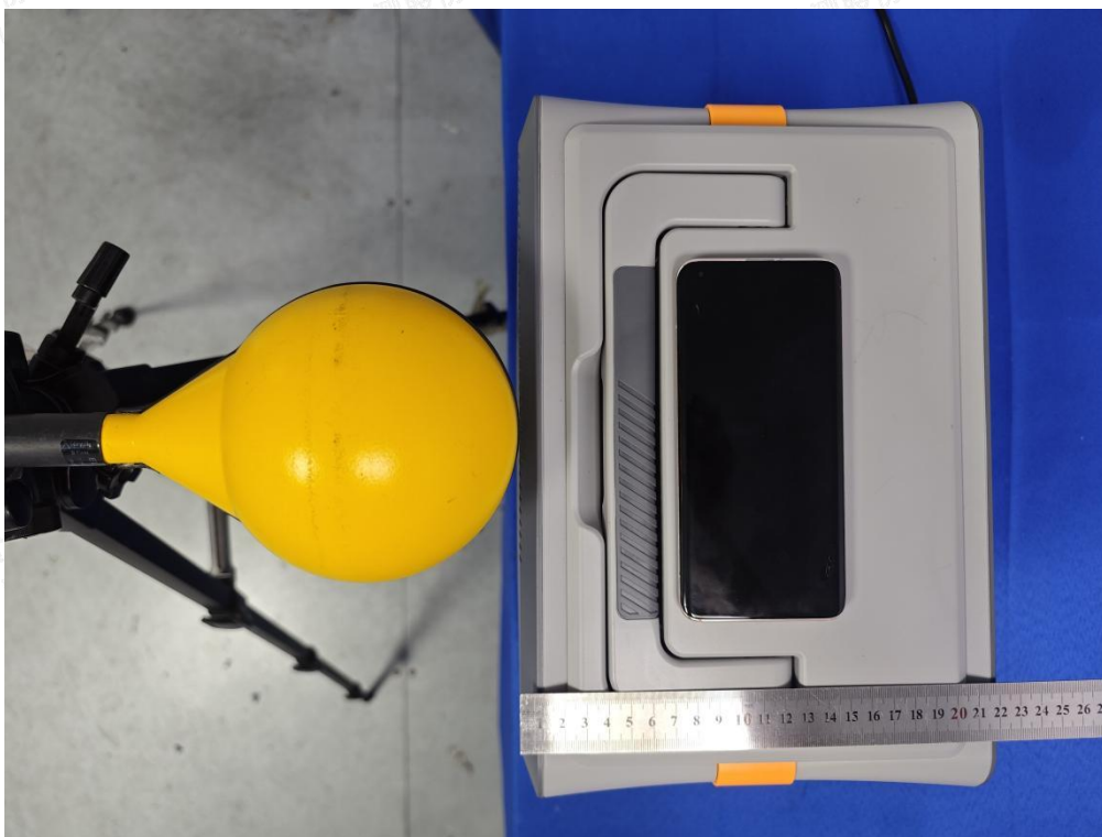
Test Position B(0cm) - Exposure photo from side edge surface-Rear(TM4)
