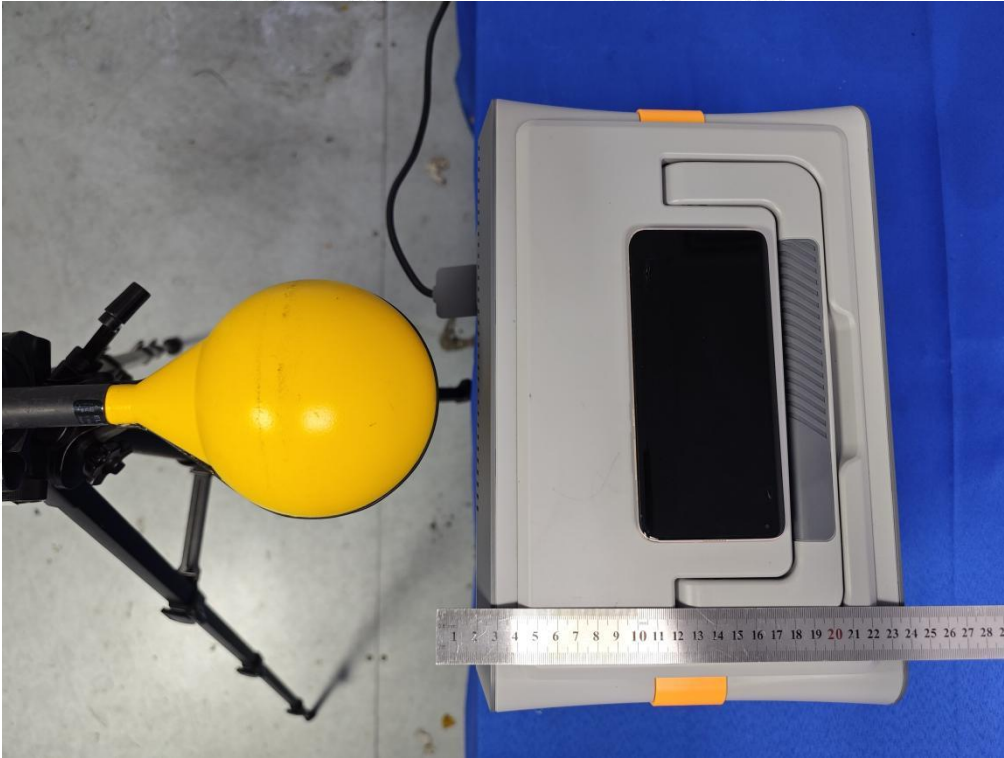
Test Position D(2cm) - Exposure photo from side edge surface-Front(TM4)
