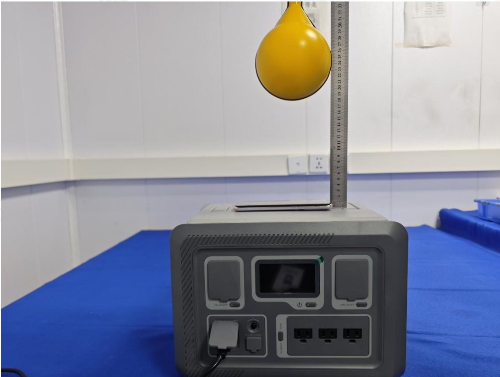
Test Position A (18cm) - Exposure photo from top surface (TM4)
