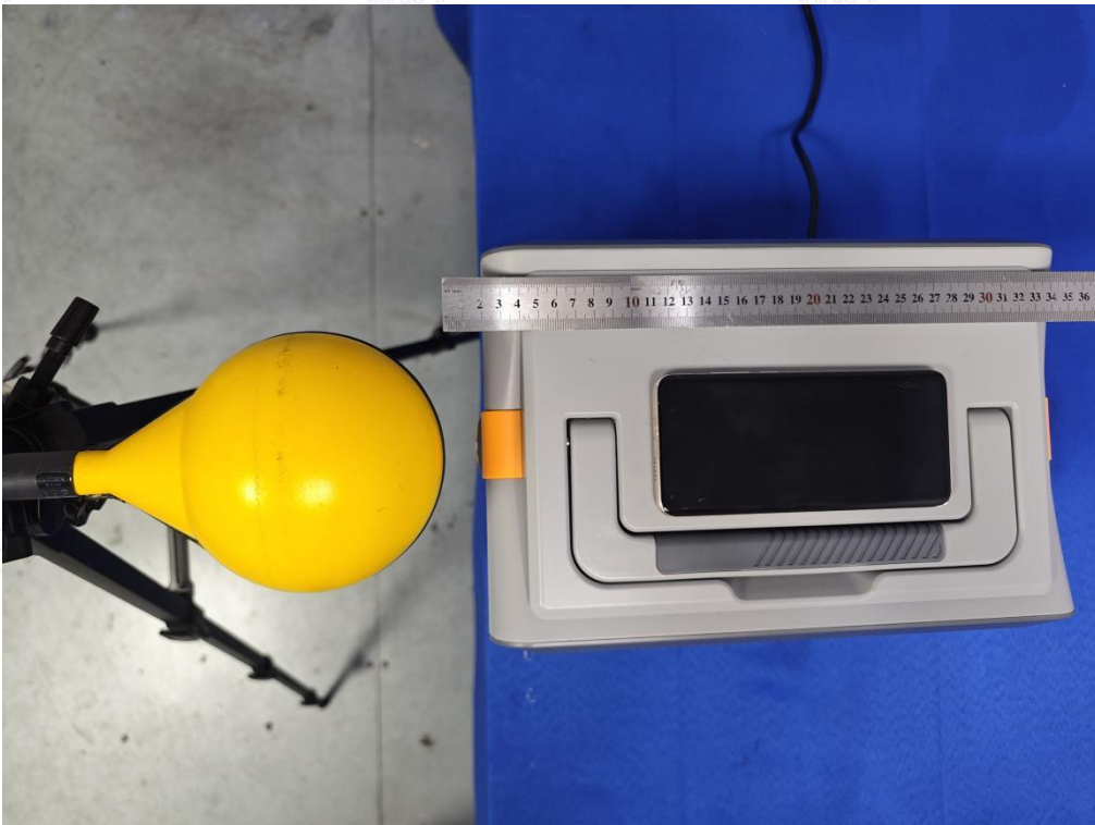
Test Position C(2cm) - Exposure photo from side edge surface-Left(TM4)
