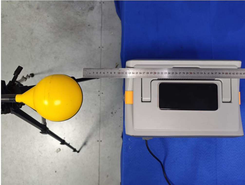
Test Position E(12cm) - Exposure photo from side edge surface-Right(TM4)
