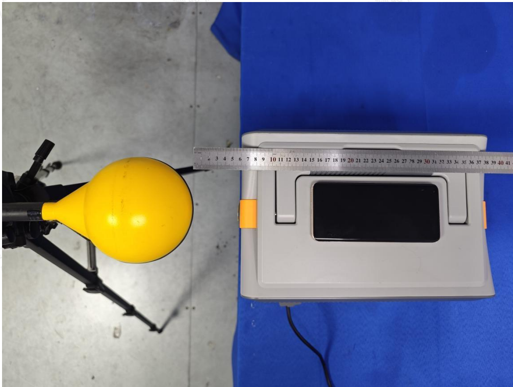
Test Position E(6cm) - Exposure photo from side edge surface-Right(TM4)
