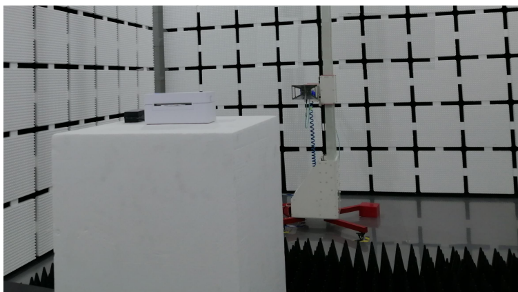
Radiated emission above 1GHz
