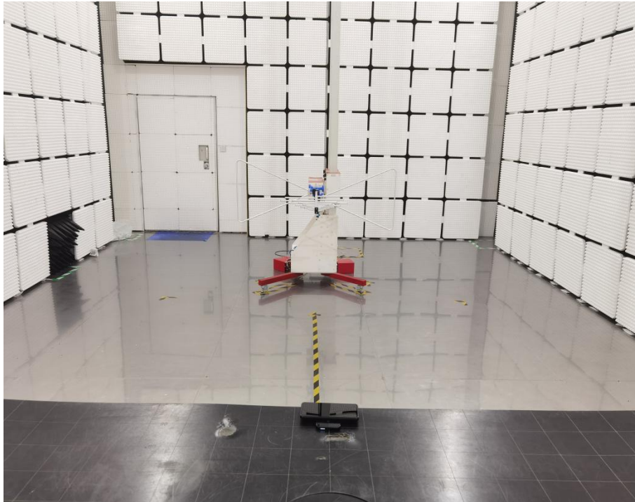
Radiated Emission (30MHz-1GHz)
