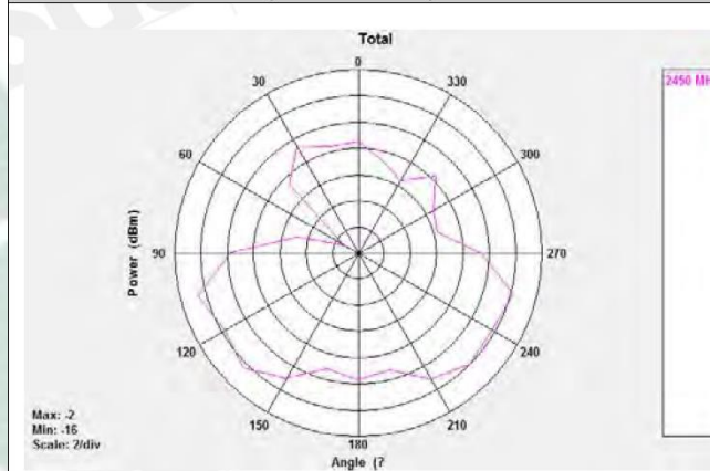
Free Space EIRP (2450 MHz) – XZ cut
