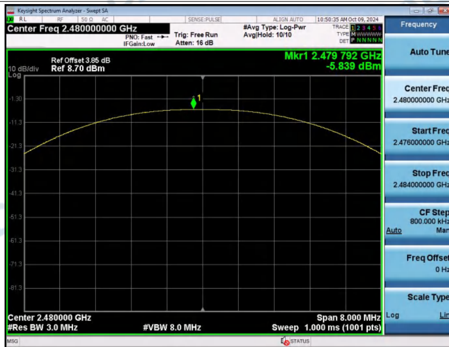
Peak_Output_Power_NVNT_ANT1_1-DH5_2480_00
