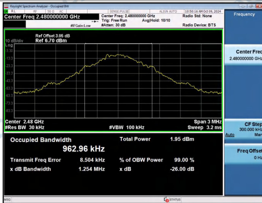
99%_Occupied_Bandwidth_NVNT_ANT1_1-DH5_2480_00
