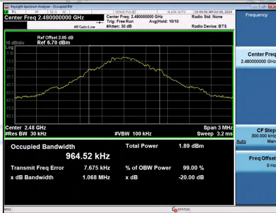
-20dB_Bandwidth_NVNT_ANT1_1-DH5_2480_00
