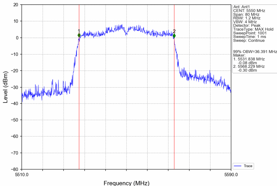
802.11n(HT40)_MCH_5550MHz_Ant1_NTNV
