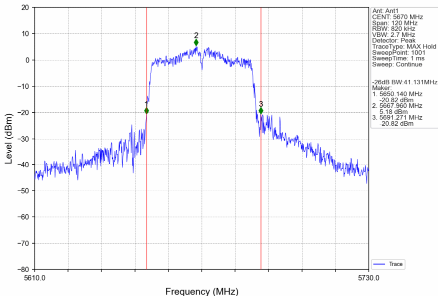
802.11n(HT40)_HCH_5670MHz_Ant1_NTNV
