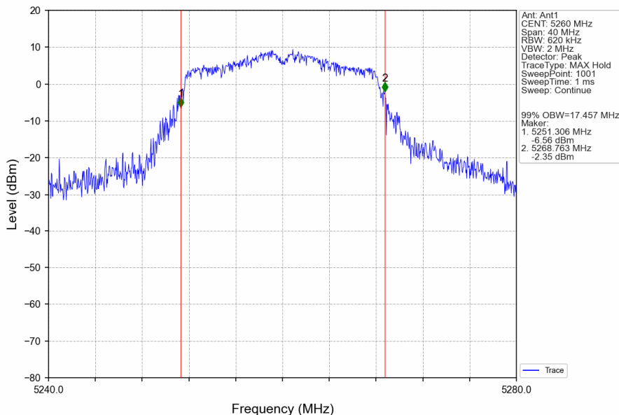
802.11a_LCH_5260MHz_Ant1_NTNV
