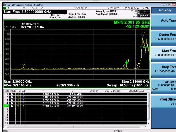
2.4G-Ant1-Hop_2405-PASS
