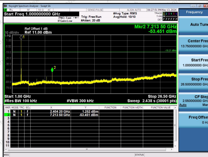
2.4G-Ant1-2405-1000~26500-PASS
