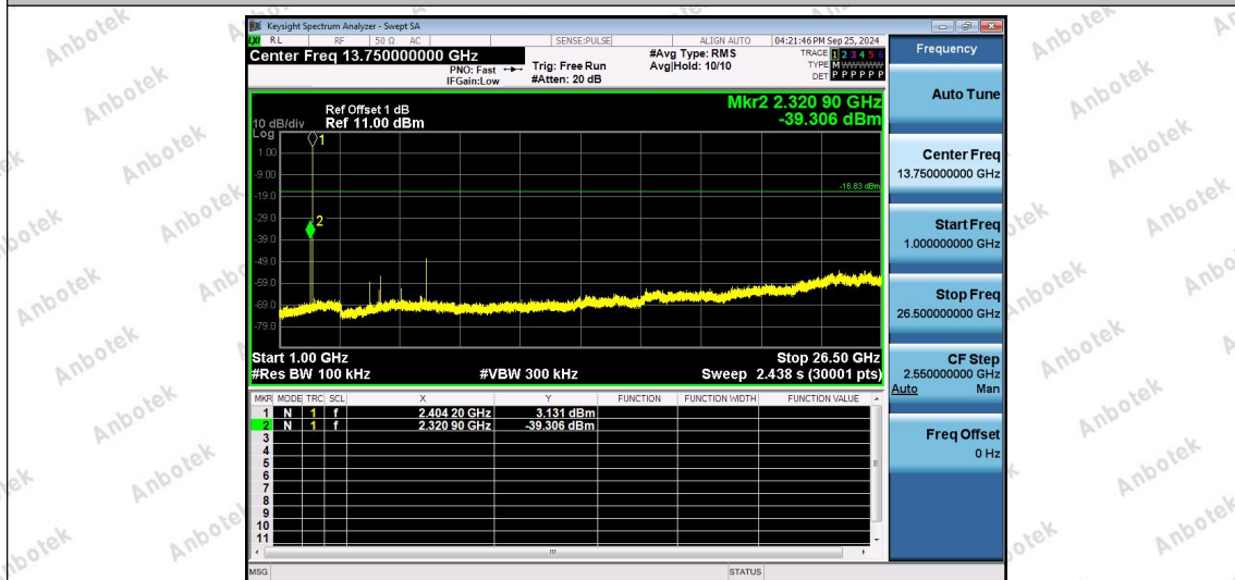
2.4G-Ant1-2405-1000~26500-PASS
