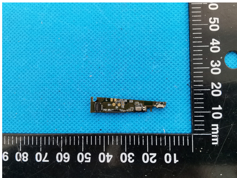
Chip Antenna
