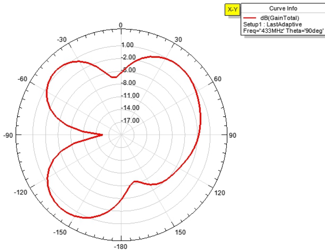
Radiation Pattern 2
