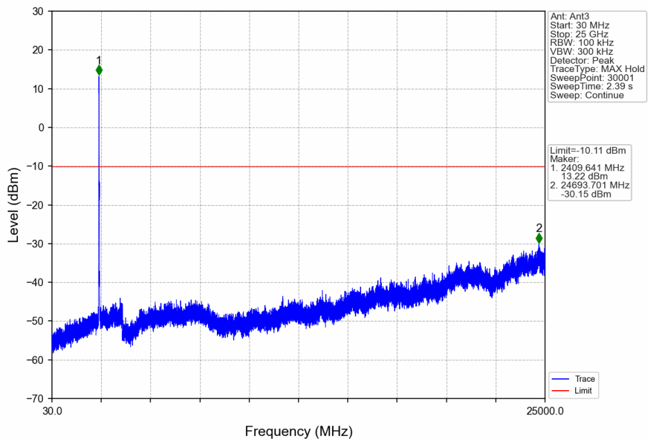
20M_LCH_2412.5MHz_Ant3_NTNV
