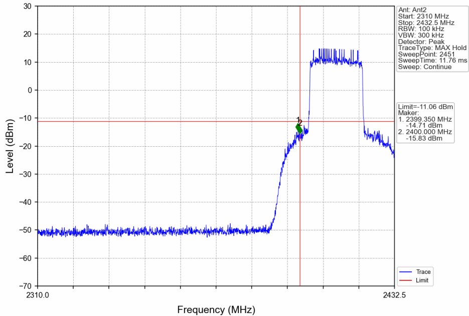
20M_LCH_2412.5MHz_Ant2_NTNV
