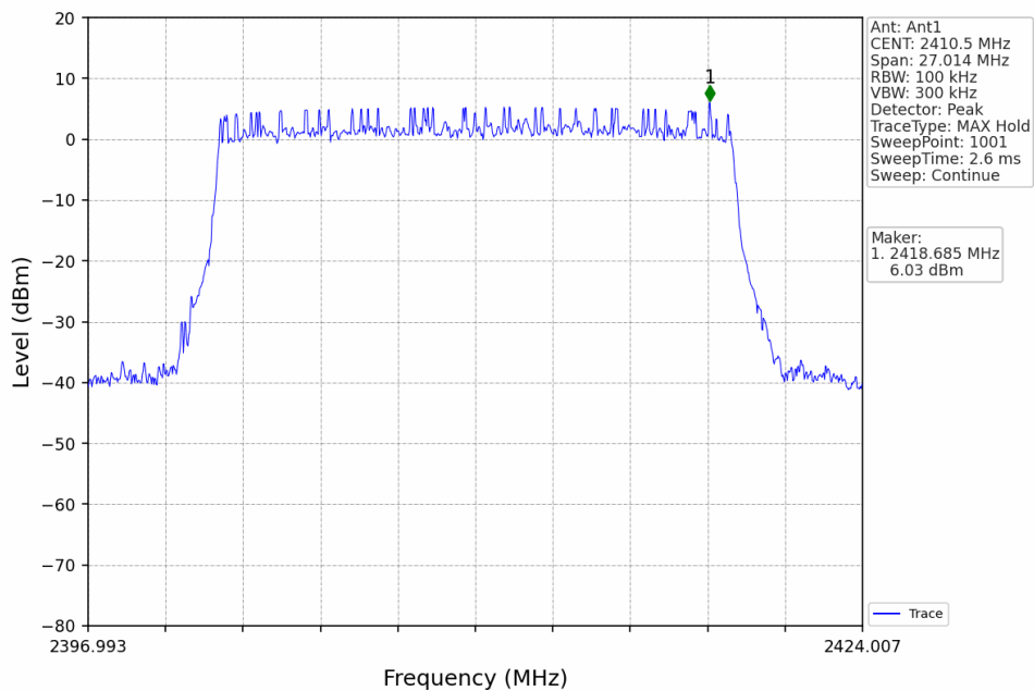
20M_LCH_2410.5MHz_Ant1_NTNV
