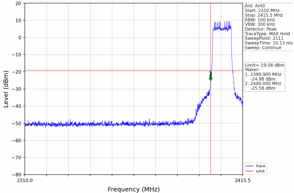
10M_LCH_2405.5MHz_Ant0_NTNV
