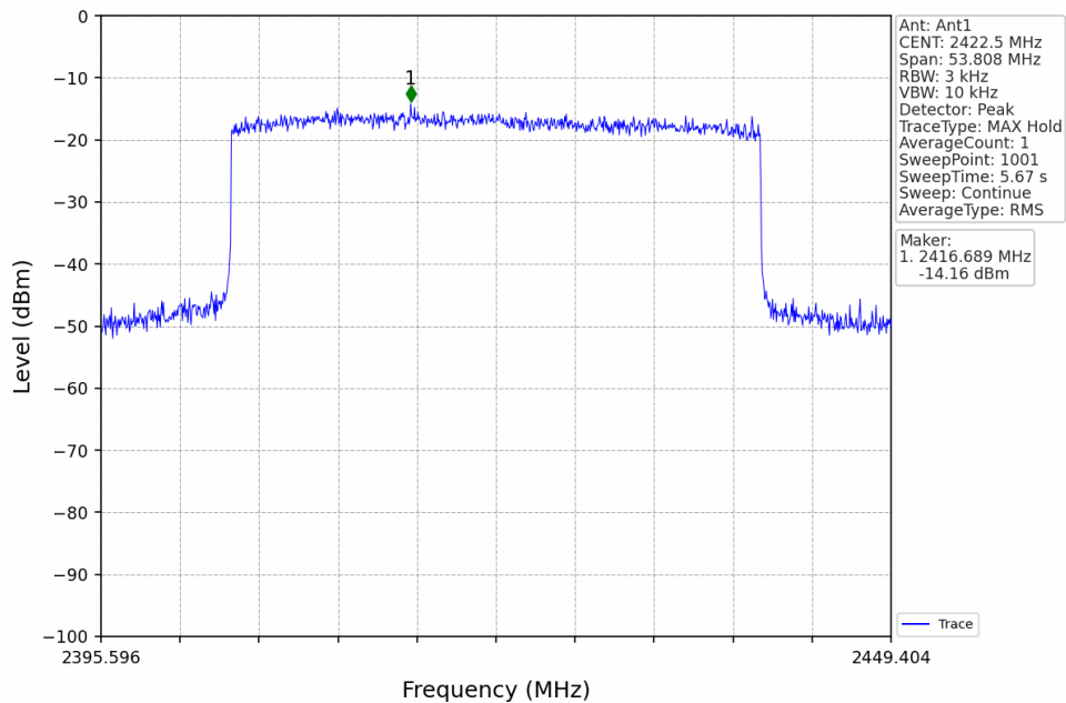
40M_LCH_2422.5MHz_Ant1_NTNV
