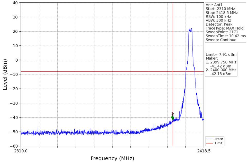
3M_LCH_2410.5MHz_Ant1_NTNV
