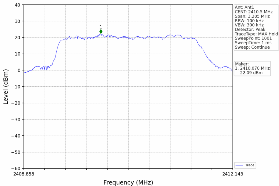
3M_LCH_2410.5MHz_Ant1_NTNV
