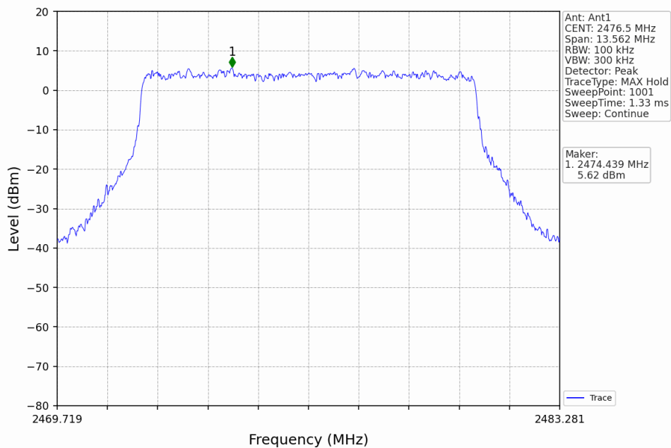
10M_HCH_2476.5MHz_Ant1_NTNV
