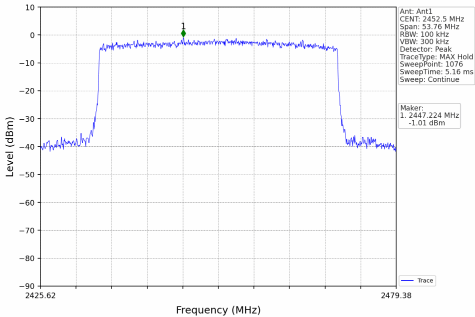
40M_HCH_2452.5MHz_Ant1_NTNV
