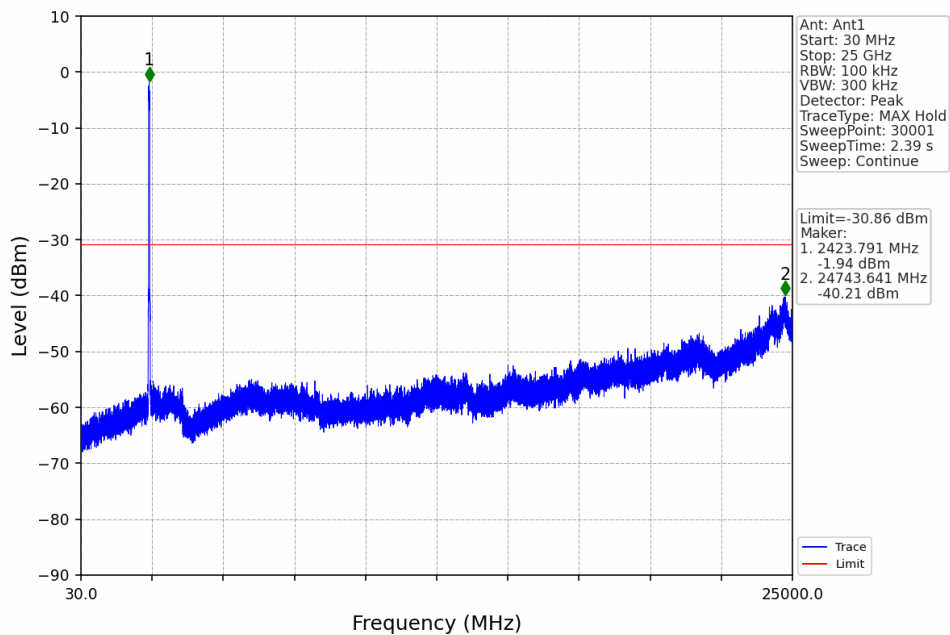
40M_LCH_2422.5MHz_Ant1_NTNV
