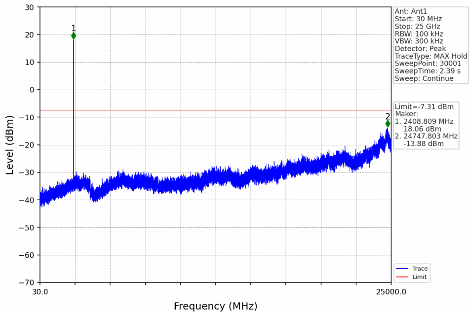
1.4M_LCH_2409.5MHz_Ant1_NTNV
