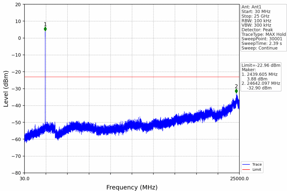
10M_MCH_2441.5MHz_Ant1_NTNV
