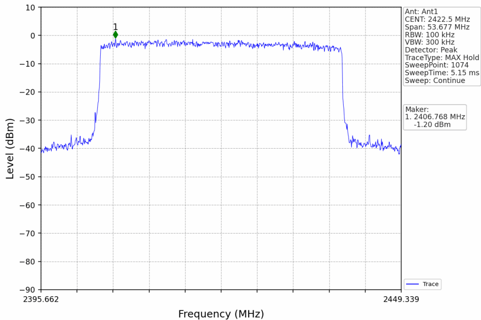
40M_LCH_2422.5MHz_Ant1_NTNV
