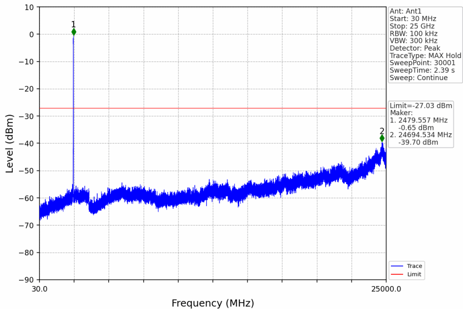
20M_HCH_2472.5MHz_Ant1_NTNV
