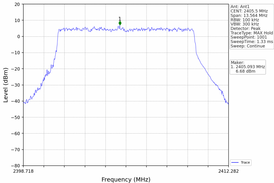
10M_LCH_2405.5MHz_Ant1_NTNV
