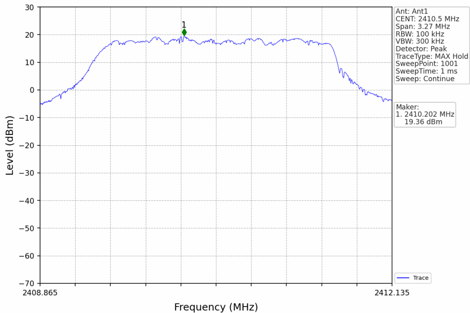
3M_LCH_2410.5MHz_Ant1_NTNV
