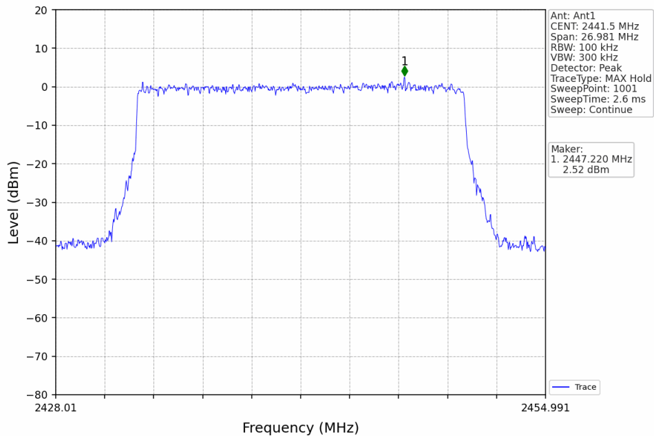
20M_MCH_2441.5MHz_Ant1_NTNV
