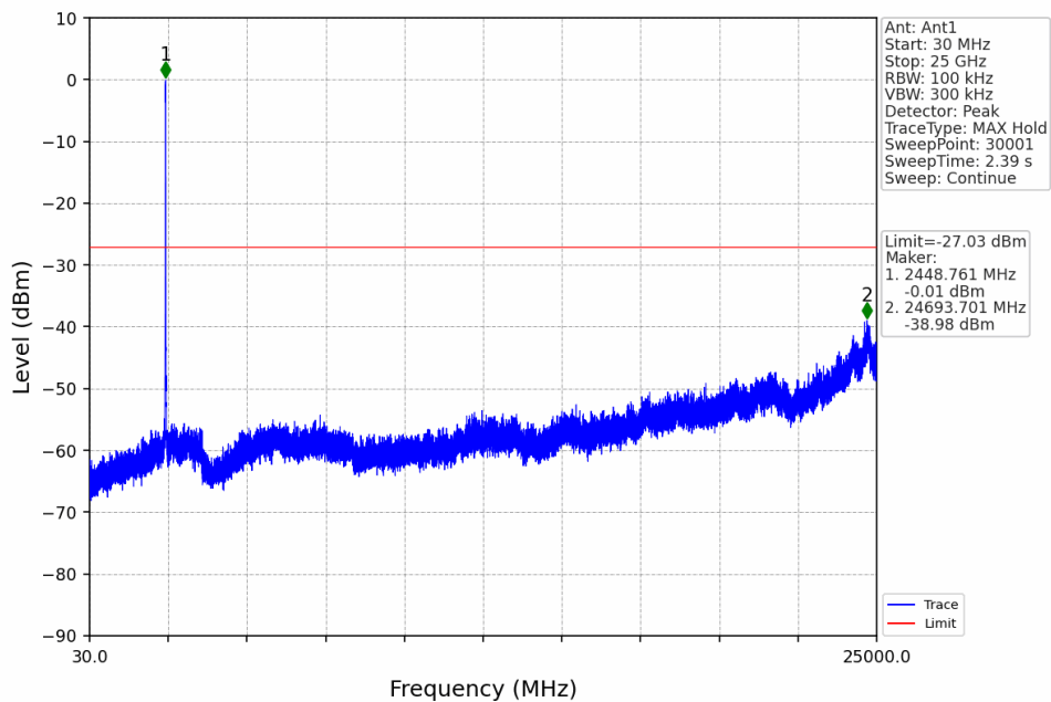
20M_MCH_2441.5MHz_Ant1_NTNV
