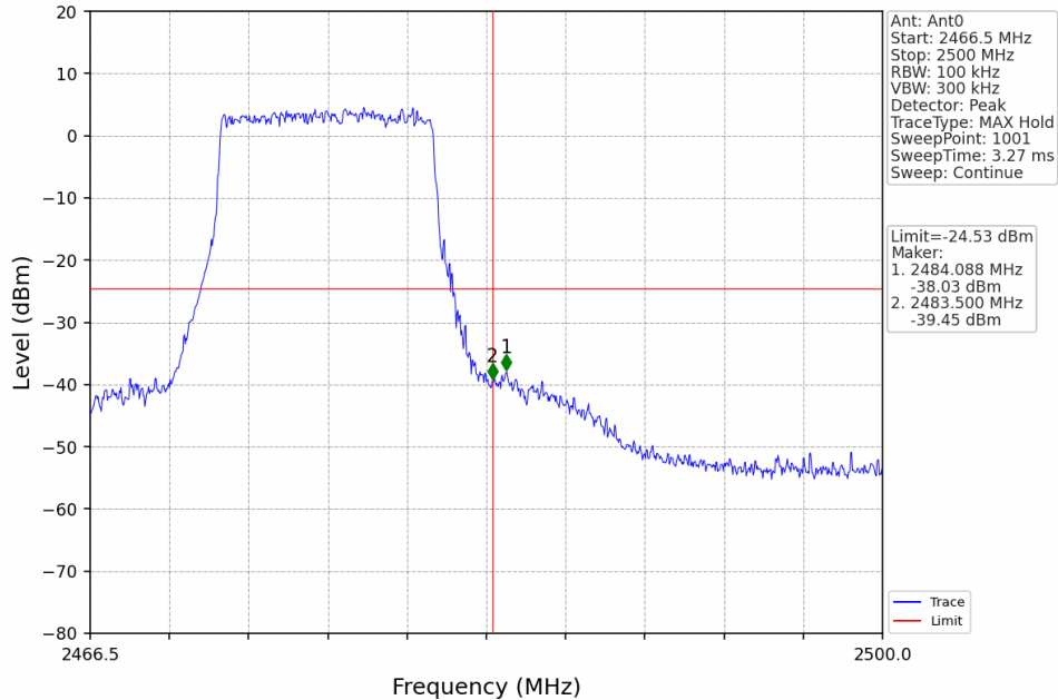
10M_HCH_2476.5MHz_Ant0_NTNV
