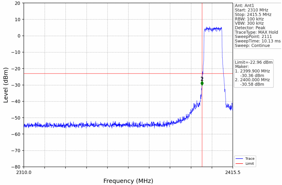
10M_LCH_2405.5MHz_Ant1_NTNV
