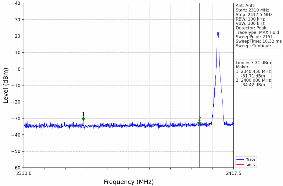
1.4M_LCH_2409.5MHz_Ant1_NTNV
