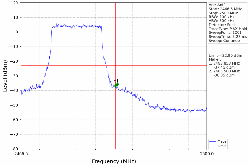
10M_HCH_2476.5MHz_Ant1_NTNV
