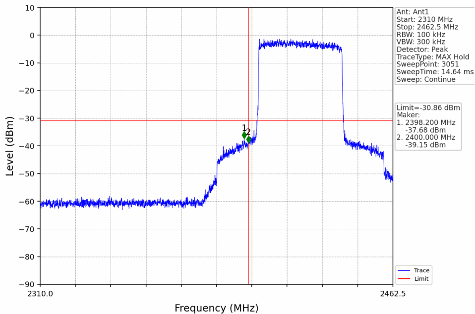
40M_LCH_2422.5MHz_Ant1_NTNV
