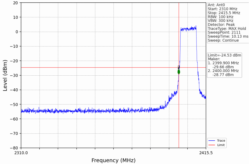
10M_LCH_2405.5MHz_Ant0_NTNV
