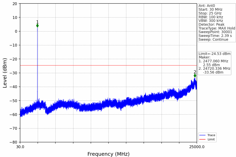
10M_HCH_2476.5MHz_Ant0_NTNV
