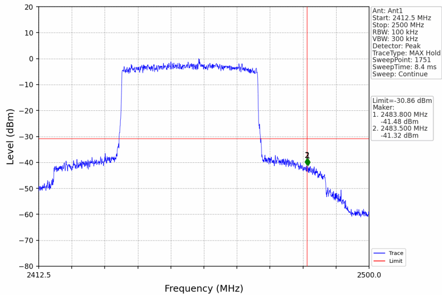
40M_HCH_2452.5MHz_Ant1_NTNV
