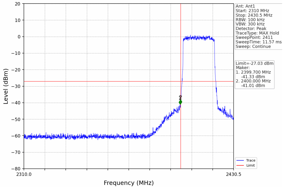
20M_LCH_2410.5MHz_Ant1_NTNV
