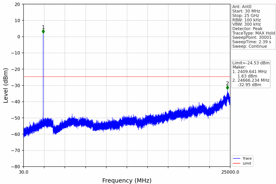
10M_LCH_2405.5MHz_Ant0_NTNV
