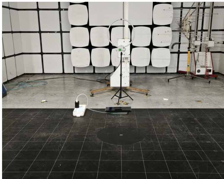
Radiated emission Below 30MHz
