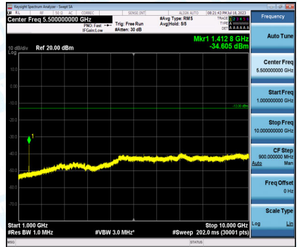
Band12-3MHz-QPSK-23095-1-0-Low-1000-10000--34.61-PASS
