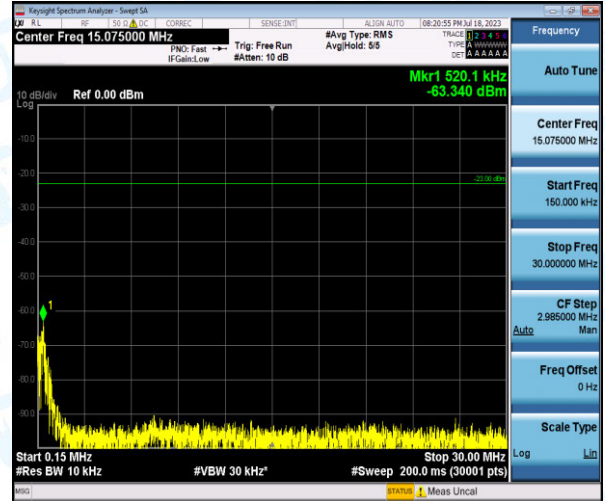
Band12-3MHz-16QAM-23025-1-0-Low-0.15-30--63.34-PASS
