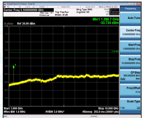
Band12-3MHz-16QAM-23025-1-0-Low-1000-10000--33.72-PASS
