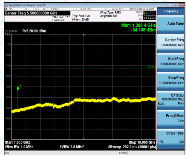
Band12-5MHz-QPSK-23035-1-0-Low-1000-10000--34.19-PASS
