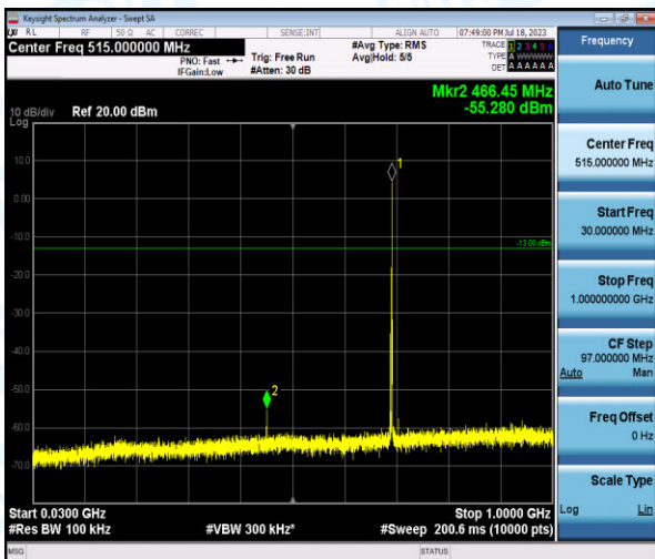
Band12-1.4MHz-16QAM-23017-1-0-Low-30-1000--55.28-PASS
