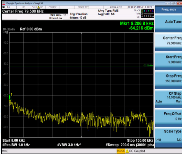
Band12-1.4MHz-16QAM-23017-1-0-Low-0.009-0.15--64.22-PASS
