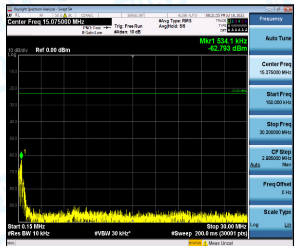
Band12-3MHz-16QAM-23095-1-0-Low-0.15-30--62.79-PASS
