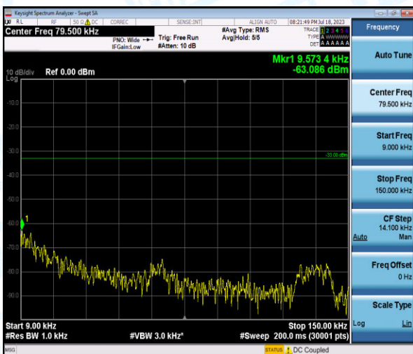
Band12-3MHz-16QAM-23095-1-0-Low-0.009-0.15--63.09-PASS
