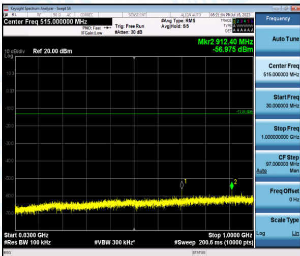
Band12-3MHz-16QAM-23025-1-0-Low-30-1000--56.98-PASS
