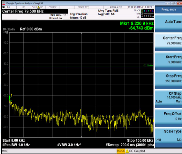
Band12-3MHz-16QAM-23025-1-0-Low-0.009-0.15--64.74-PASS
