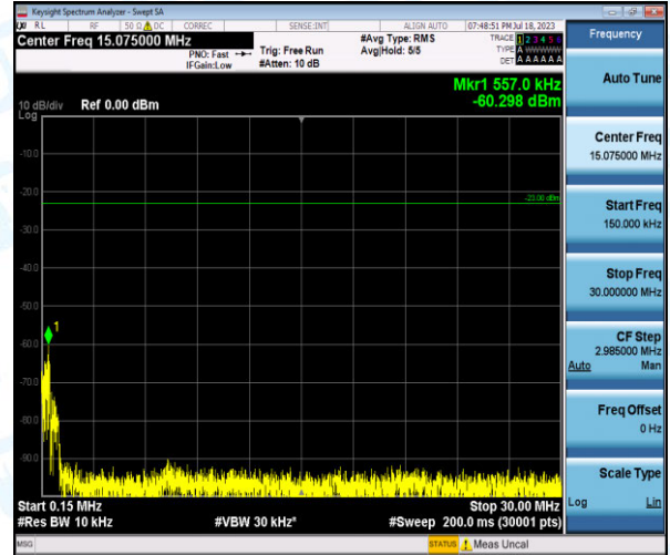
Band12-1.4MHz-16QAM-23017-1-0-Low-0.15-30--60.3-PASS
