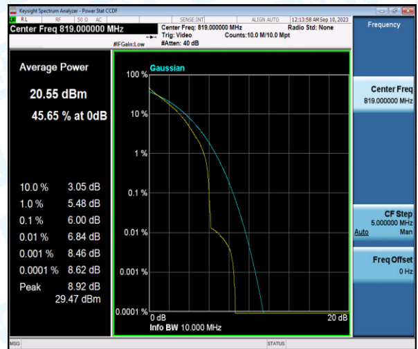
Band26-3MHz-16QAM-26740-6-0-Low-6.00-<=13-PASS
