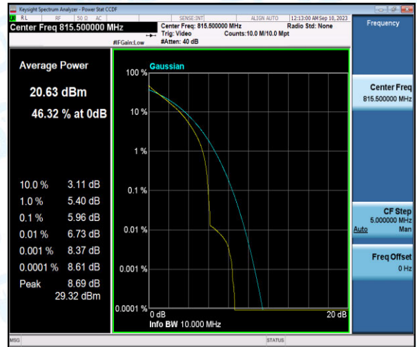
Band26-3MHz-16QAM-26705-6-0-Low-5.96-<=13-PASS
