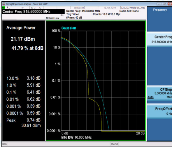
Band26-3MHz-16QAM-26705-1-0-Low-6.41-<=13-PASS
