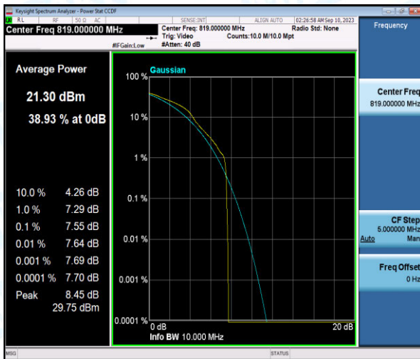
Band26-5MHz-16QAM-26740-1-0-Low-7.55-<=13-PASS
