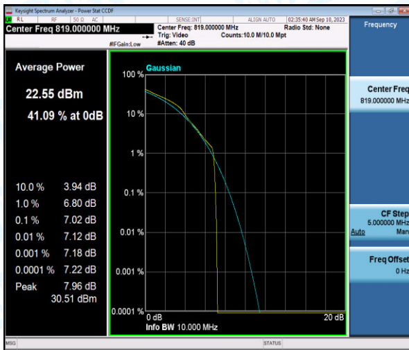
Band26-10MHz-16QAM-26740-1-0-Low-7.02-<=13-PASS
