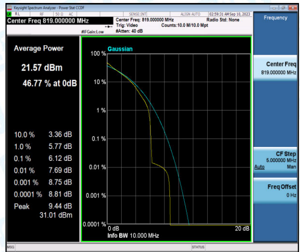
Band26-10MHz-16QAM-26740-6-0-Low-6.12-<=13-PASS
