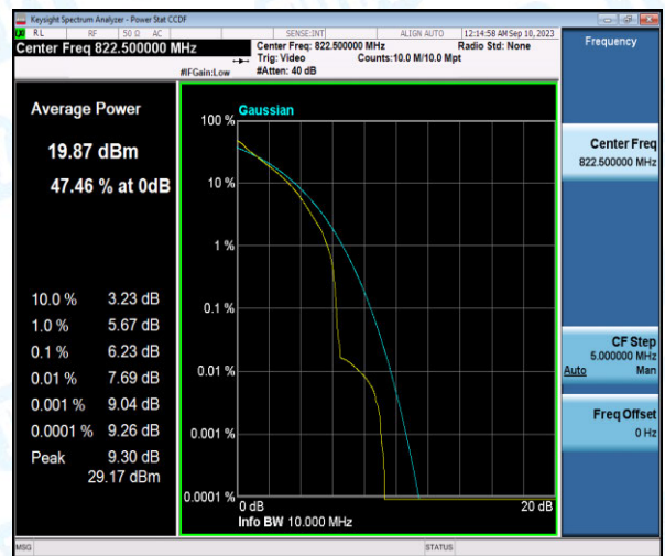
Band26-3MHz-16QAM-26775-6-0-High-6.23-<=13-PASS
