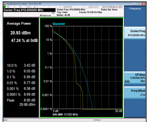
Band26-5MHz-16QAM-26740-6-0-Low-6.56-<=13-PASS
