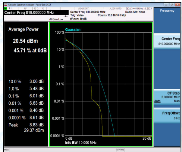
Band26-3MHz-QPSK-26740-6-0-Low-6.01-<=13-PASS
