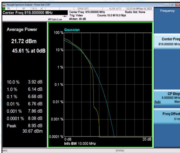
Band26-3MHz-QPSK-26740-1-0-Low-6.68-<=13-PASS
