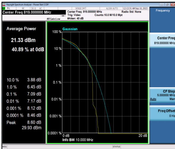
Band26-3MHz-16QAM-26740-1-0-Low-7.09-<=13-PASS
