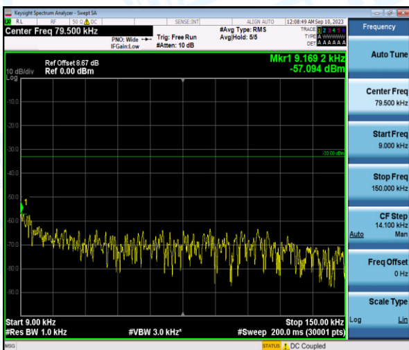
Band26-1.4MHz-16QAM-26740-1-0-Low-0.009-0.15--57.09-PASS
