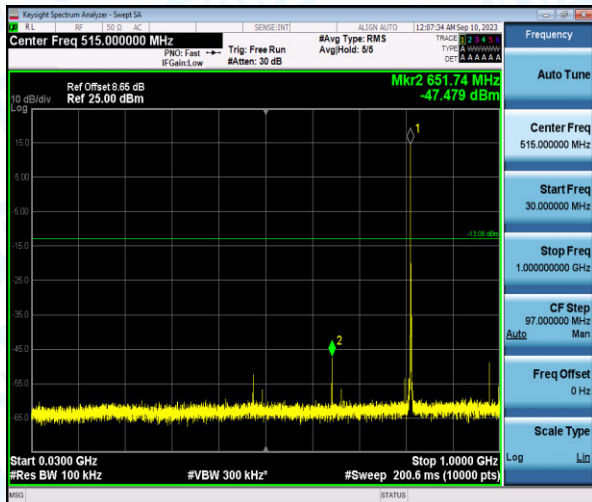
Band26-1.4MHz-QPSK-26697-1-0-Low-30-1000--47.48-PASS
