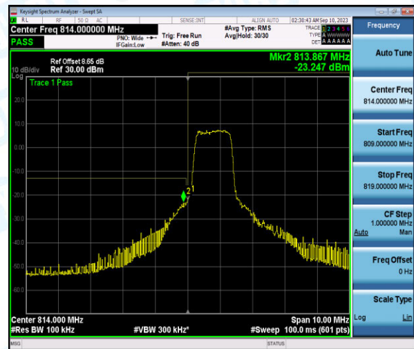
Band26-5MHz-QPSK-26715-6-0-Low--22.20,-23.25-PASS
