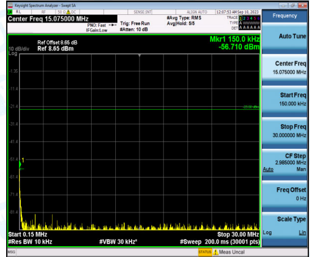
Band26-1.4MHz-16QAM-26697-1-0-Low-0.15-30--56.71-PASS
