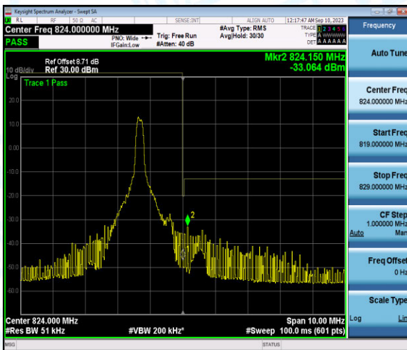
Band26-3MHz-QPSK-26775-1-0-High--47.21,-33.06-PASS
