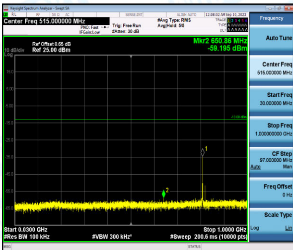
Band26-1.4MHz-16QAM-26697-1-0-Low-30-1000--59.2-PASS
