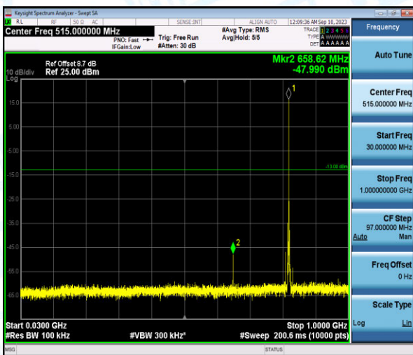
Band26-1.4MHz-QPSK-26783-1-0-High-30-1000--47.99-PASS
