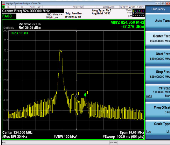
Band26-1.4MHz-QPSK-26783-1-0-High--38.42,-37.28-PASS
