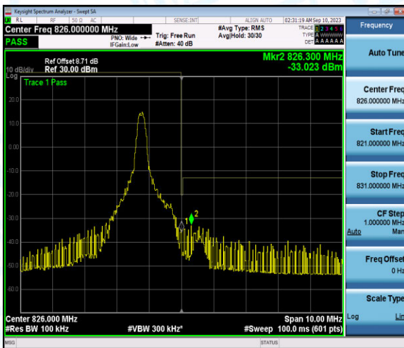
Band26-5MHz-16QAM-26785-1-0-High--36.18,-33.02-PASS
