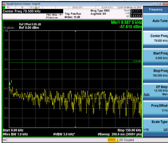
Band26-1.4MHz-QPSK-26697-1-0-Low-0.009-0.15--57.61-PASS
