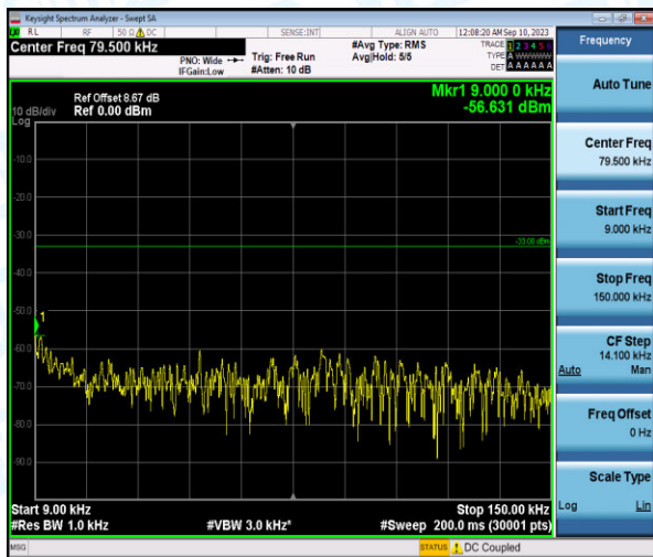
Band26-1.4MHz-QPSK-26740-1-0-Low-0.009-0.15--56.63-PASS
