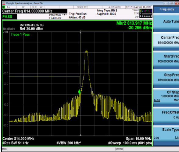
Band26-3MHz-16QAM-26705-1-0-Low--28.89,-30.27-PASS
