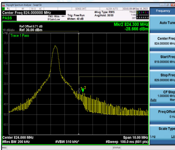
Band26-10MHz-16QAM-26740-1-0-High--29.33,-28.67-PASS
