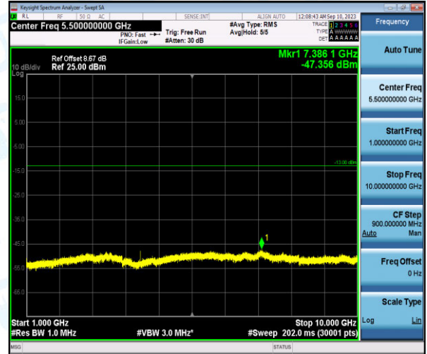
Band26-1.4MHz-QPSK-26740-1-0-Low-1000-10000--47.36-PASS
