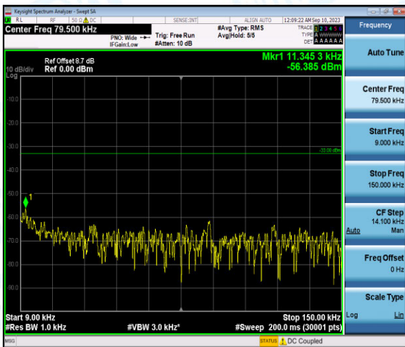
Band26-1.4MHz-QPSK-26783-1-0-High-0.009-0.15--56.39-PASS
