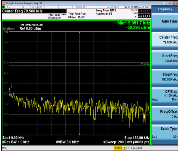
Band26-1.4MHz-16QAM-26697-1-0-Low-0.009-0.15--58.29-PASS
