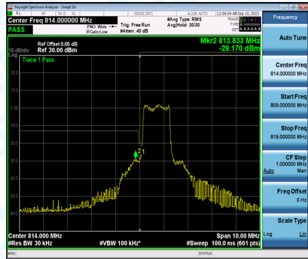
Band26-1.4MHz-QPSK-26697-6-0-Low--29.87,-29.17-PASS
