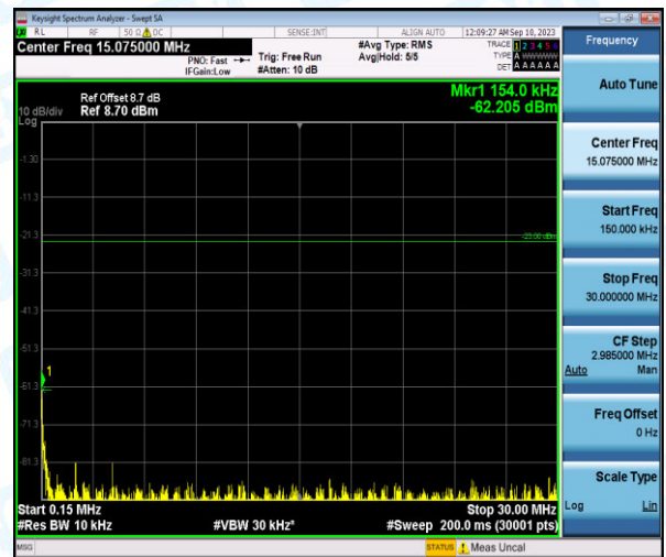
Band26-1.4MHz-QPSK-26783-1-0-High-0.15-30--62.21-PASS
