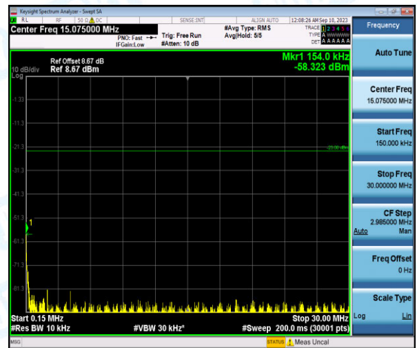
Band26-1.4MHz-QPSK-26740-1-0-Low-0.15-30--58.32-PASS
