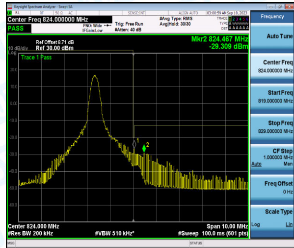
Band26-10MHz-QPSK-26740-1-0-High--26.75,-29.31-PASS
