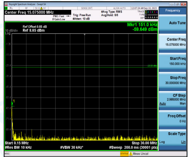
Band26-1.4MHz-QPSK-26697-1-0-Low-0.15-30--59.65-PASS
