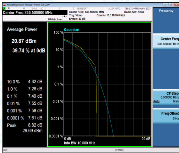
Band26-5MHz-16QAM-26915-1-0-Low-7.49-<=13-PASS
