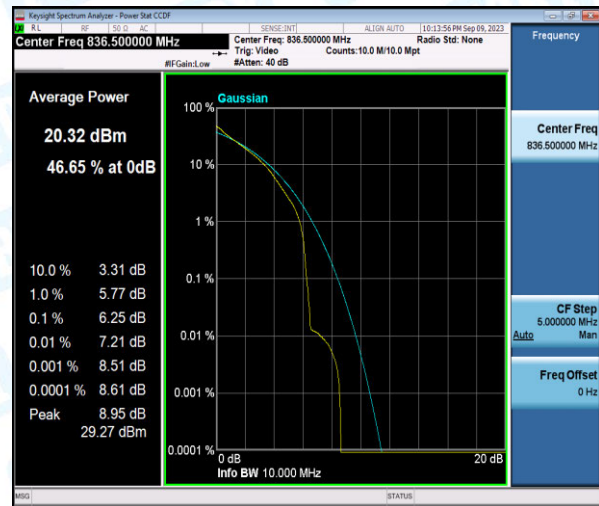
Band26-5MHz-16QAM-26915-6-0-Low-6.25-<=13-PASS
