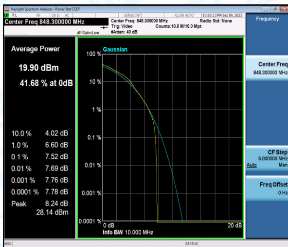
Band26-1.4MHz-16QAM-27033-1-0-High-7.52-<=13-PASS
