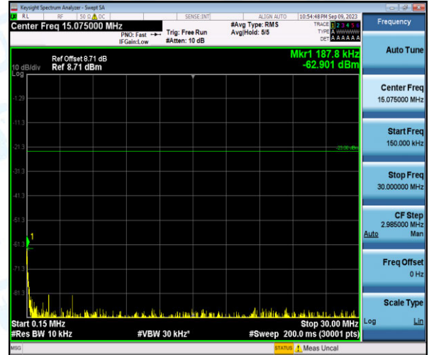
Band26-3MHz-16QAM-26805-1-0-Low-0.15-30--62.9-PASS
