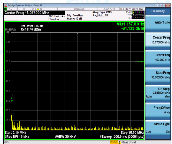
Band26-5MHz-QPSK-26915-1-0-Low-0.15-30--61.13-PASS
