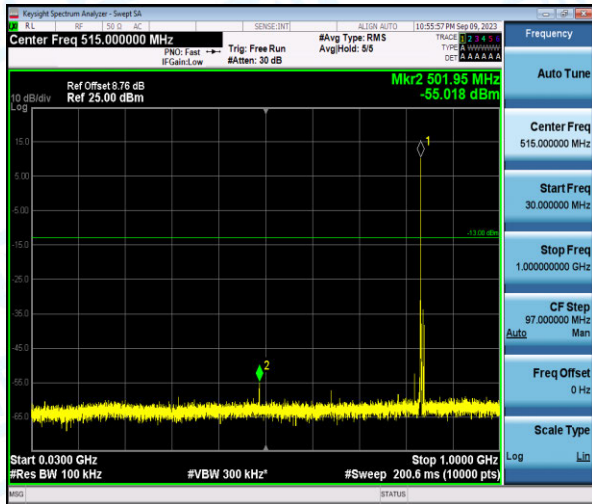
Band26-3MHz-16QAM-26915-1-0-Low-30-1000--55.02-PASS
