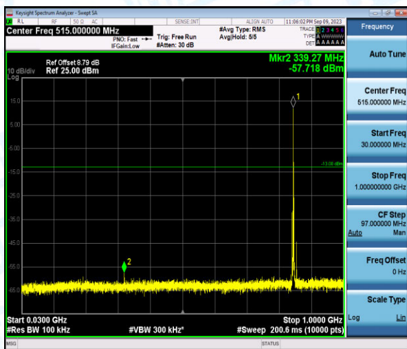
Band26-5MHz-QPSK-27015-1-0-High-30-1000--57.72-PASS
