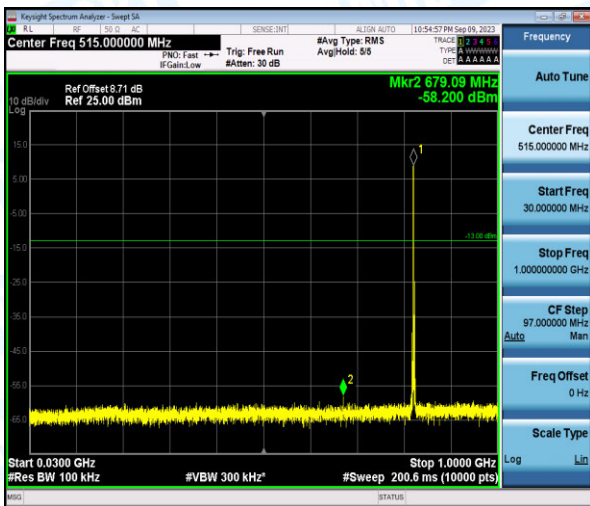
Band26-3MHz-16QAM-26805-1-0-Low-30-1000--58.2-PASS
