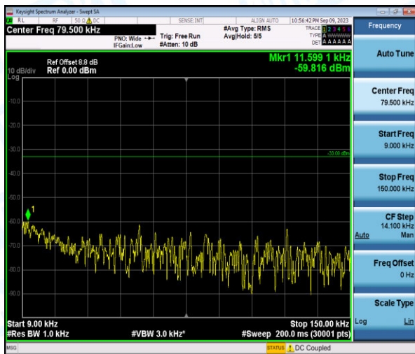
Band26-3MHz-16QAM-27025-1-0-High-0.009-0.15--59.82-PASS
