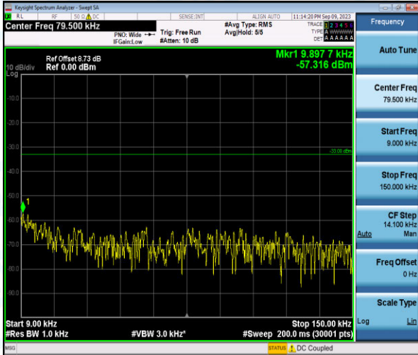
Band26-10MHz-16QAM-26840-1-0-Low-0.009-0.15--57.32-PASS
