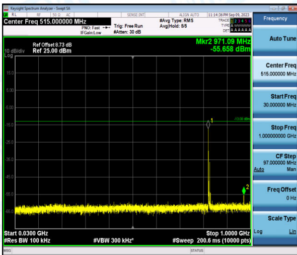
Band26-10MHz-16QAM-26840-1-0-Low-30-1000--55.66-PASS
