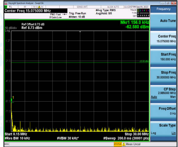
Band26-10MHz-QPSK-26840-1-0-Low-0.15-30--62.58-PASS
