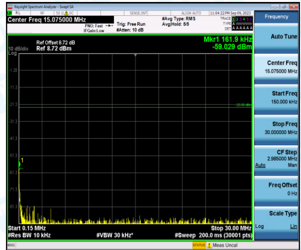
Band26-5MHz-16QAM-26815-1-0-Low-0.15-30--59.03-PASS
