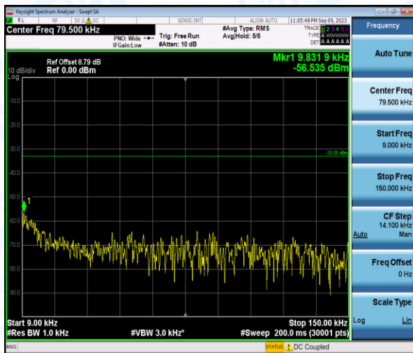
Band26-5MHz-QPSK-27015-1-0-High-0.009-0.15--56.54-PASS
