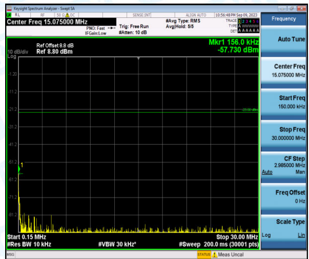
Band26-3MHz-16QAM-27025-1-0-High-0.15-30--57.73-PASS
