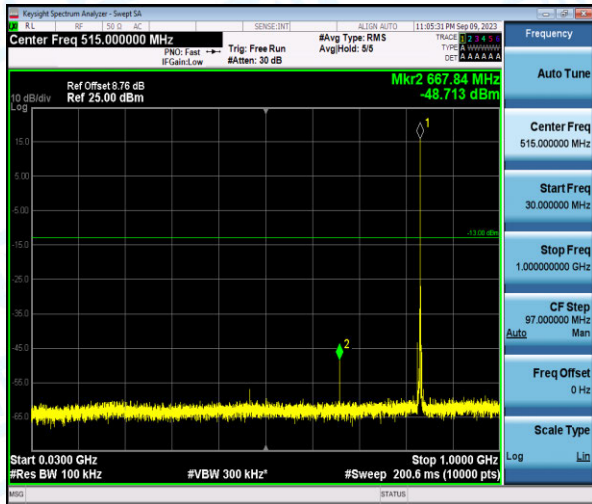
Band26-5MHz-16QAM-26915-1-0-Low-30-1000--48.71-PASS
