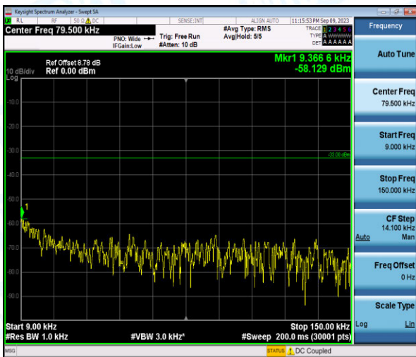
Band26-10MHz-QPSK-26990-1-0-High-0.009-0.15--58.13-PASS
