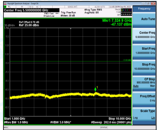
Band26-5MHz-16QAM-26915-1-0-Low-1000-10000--47.14-PASS
