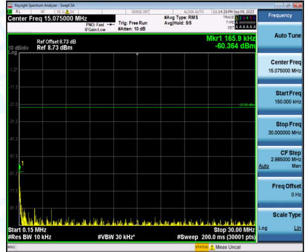
Band26-10MHz-16QAM-26840-1-0-Low-0.15-30--60.36-PASS
