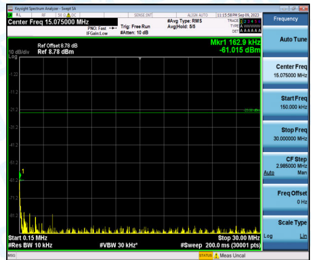
Band26-10MHz-QPSK-26990-1-0-High-0.15-30--61.02-PASS
