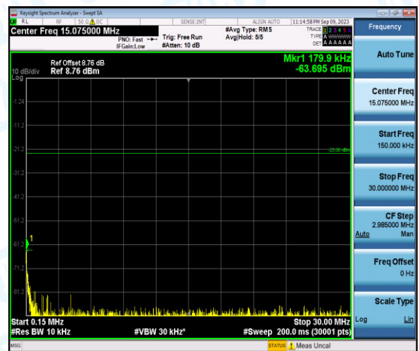
Band26-10MHz-QPSK-26915-1-0-Low-0.15-30--63.7-PASS
