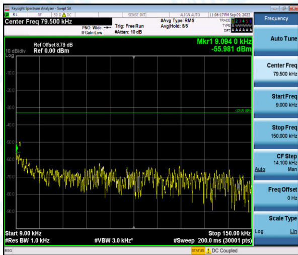
Band26-5MHz-16QAM-27015-1-0-High-0.009-0.15--55.98-PASS
