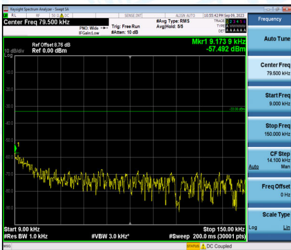
Band26-3MHz-16QAM-26915-1-0-Low-0.009-0.15--57.49-PASS
