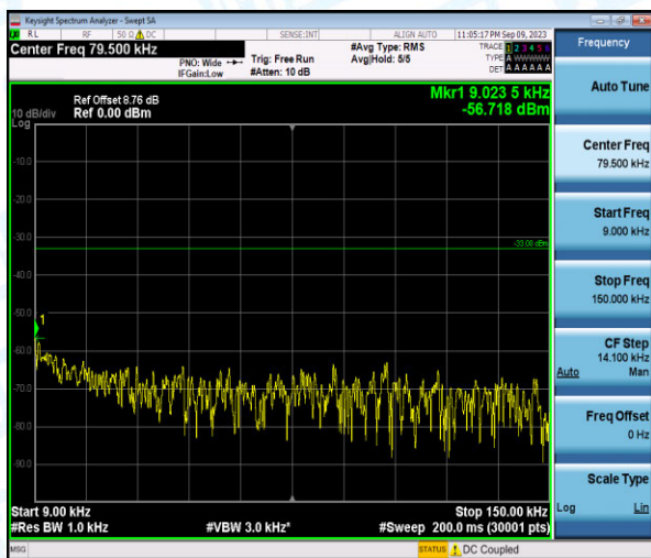
Band26-5MHz-16QAM-26915-1-0-Low-0.009-0.15--56.72-PASS
