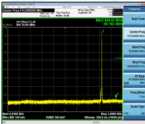
Band26-5MHz-QPSK-26815-1-0-Low-30-1000--59.16-PASS
