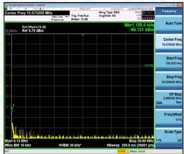
Band26-5MHz-QPSK-27015-1-0-High-0.15-30--65.13-PASS
