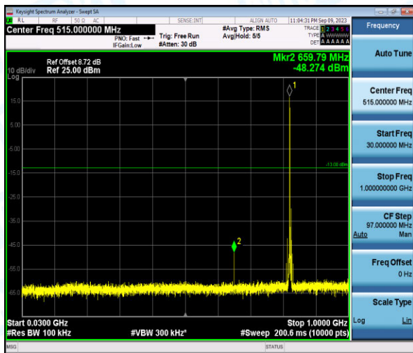
Band26-5MHz-16QAM-26815-1-0-Low-30-1000--48.27-PASS
