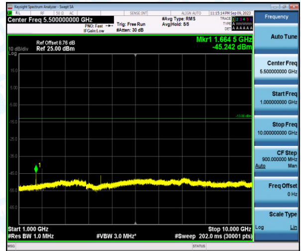
Band26-10MHz-QPSK-26915-1-0-Low-1000-10000--45.24-PASS
