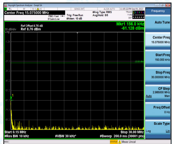
Band26-5MHz-16QAM-26915-1-0-Low-0.15-30--61.13-PASS
