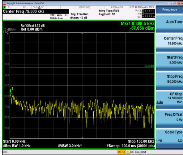
Band26-5MHz-QPSK-26815-1-0-Low-0.009-0.15--57.66-PASS
