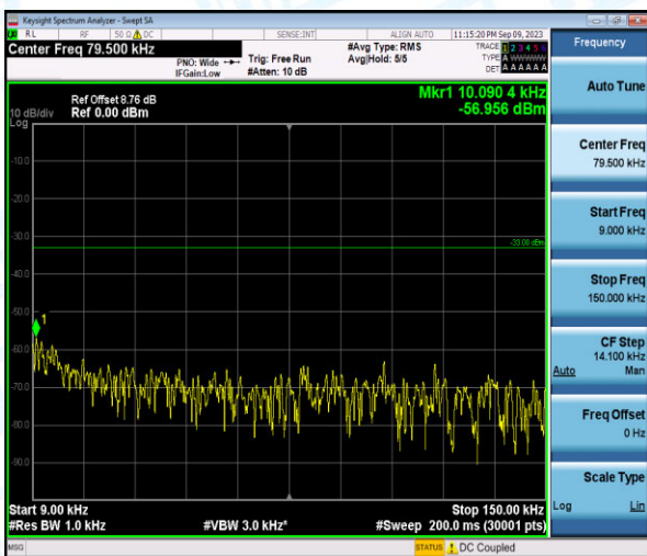
Band26-10MHz-16QAM-26915-1-0-Low-0.009-0.15--56.96-PASS
