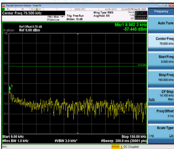
Band26-10MHz-QPSK-26915-1-0-Low-0.009-0.15--57.45-PASS
