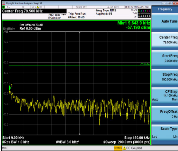
Band26-10MHz-QPSK-26840-1-0-Low-0.009-0.15--57.19-PASS
