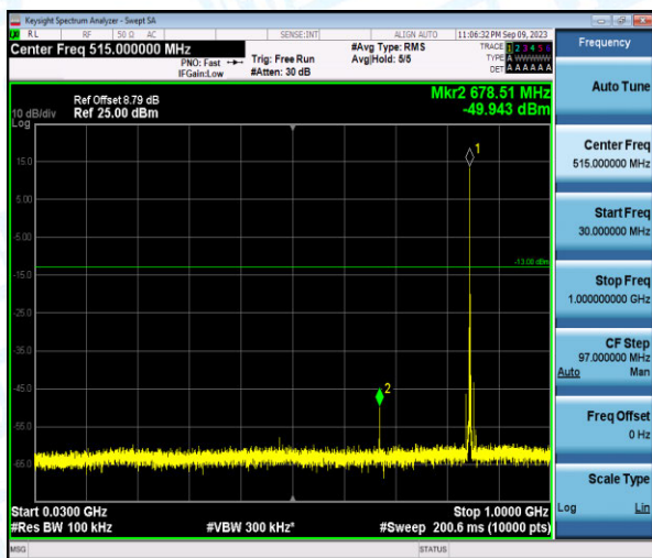
Band26-5MHz-16QAM-27015-1-0-High-30-1000--49.94-PASS
