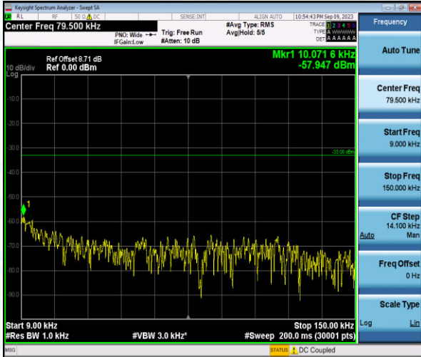
Band26-3MHz-16QAM-26805-1-0-Low-0.009-0.15--57.95-PASS
