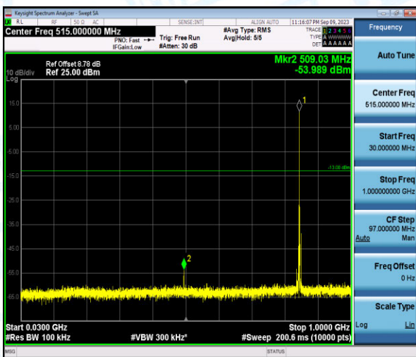
Band26-10MHz-QPSK-26990-1-0-High-30-1000--53.99-PASS
