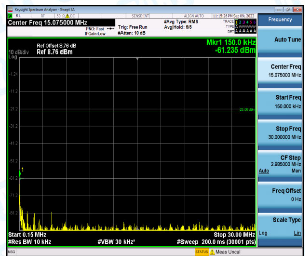
Band26-10MHz-16QAM-26915-1-0-Low-0.15-30--61.24-PASS
