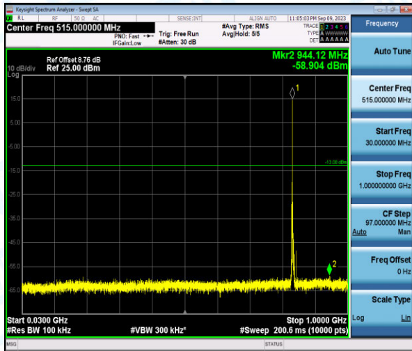
Band26-5MHz-QPSK-26915-1-0-Low-30-1000--58.9-PASS
