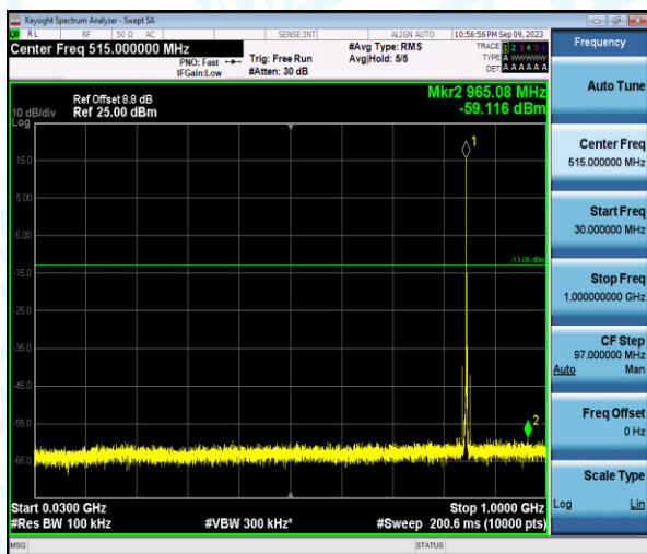
Band26-3MHz-16QAM-27025-1-0-High-30-1000--59.12-PASS
