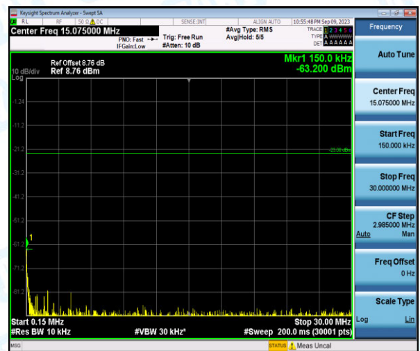
Band26-3MHz-16QAM-26915-1-0-Low-0.15-30--63.2-PASS
