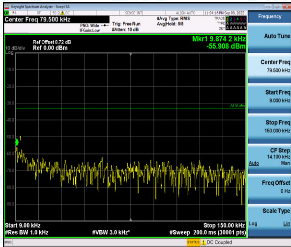
Band26-5MHz-16QAM-26815-1-0-Low-0.009-0.15--55.91-PASS
