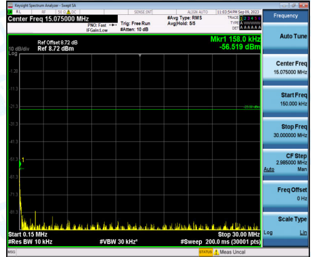
Band26-5MHz-QPSK-26815-1-0-Low-0.15-30--56.52-PASS
