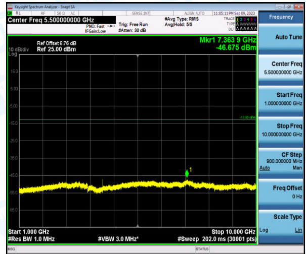
Band26-5MHz-QPSK-26915-1-0-Low-1000-10000--46.68-PASS
