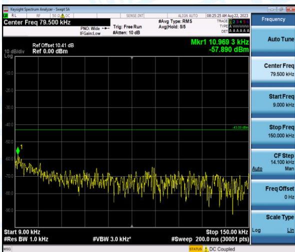
Band4-5MHz-QPSK-20175-1-0-Low-0.009-0.15--57.89-PASS
