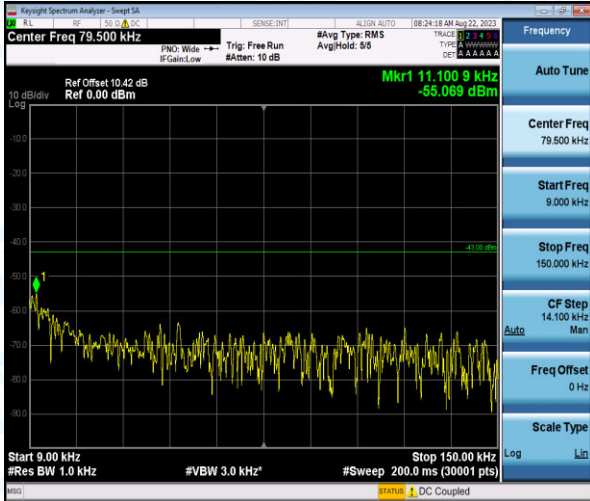
Band4-5MHz-QPSK-19975-1-0-Low-0.009-0.15--55.07-PASS
