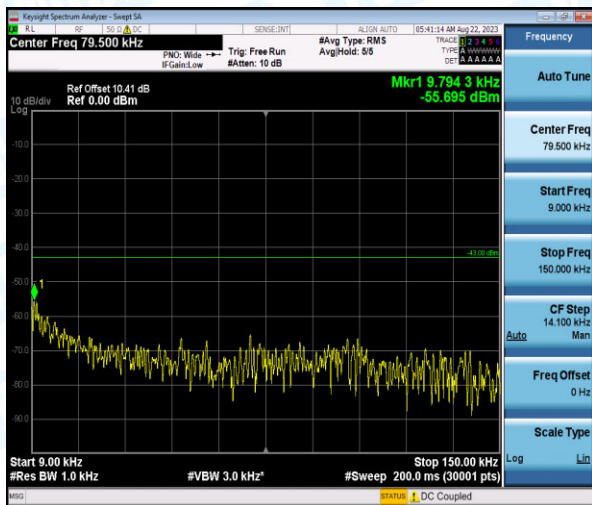
Band4-1.4MHz-QPSK-20175-1-0-Low-0.009-0.15--55.7-PASS
