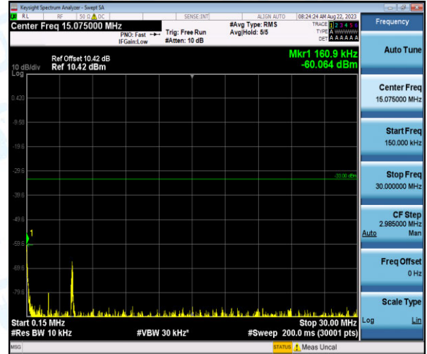
Band4-5MHz-QPSK-19975-1-0-Low-0.15-30--60.06-PASS
