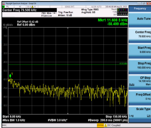
Band4-1.4MHz-QPSK-19957-1-0-Low-0.009-0.15--58.5-PASS
