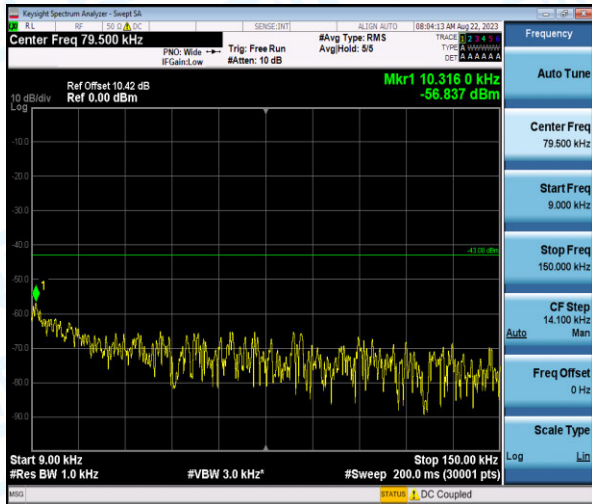
Band4-3MHz-16QAM-19965-1-0-Low-0.009-0.15--56.84-PASS
