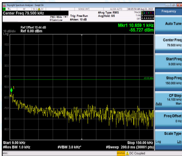
Band4-3MHz-QPSK-20385-1-0-High-0.009-0.15--55.73-PASS
