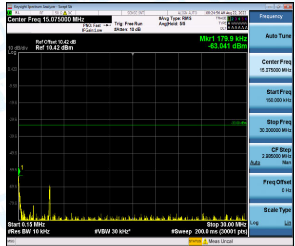
Band4-5MHz-16QAM-19975-1-0-Low-0.15-30--63.04-PASS
