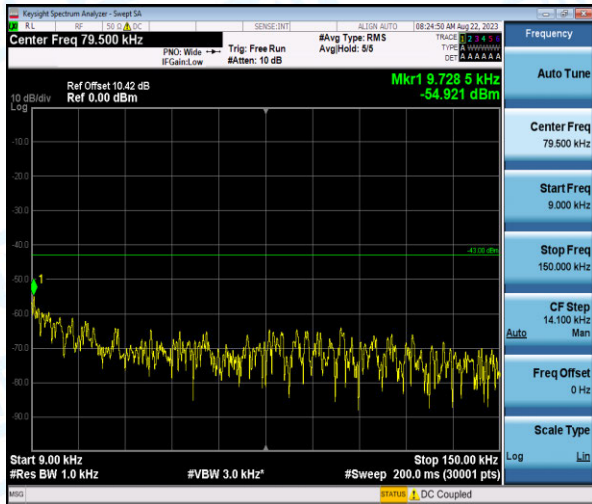
Band4-5MHz-16QAM-19975-1-0-Low-0.009-0.15--54.92-PASS
