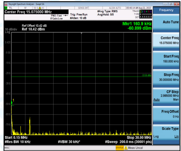
Band4-1.4MHz-QPSK-19957-1-0-Low-0.15-30--60.9-PASS
