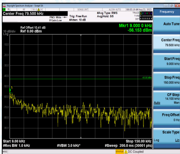
Band4-3MHz-16QAM-20175-1-0-Low-0.009-0.15--56.15-PASS
