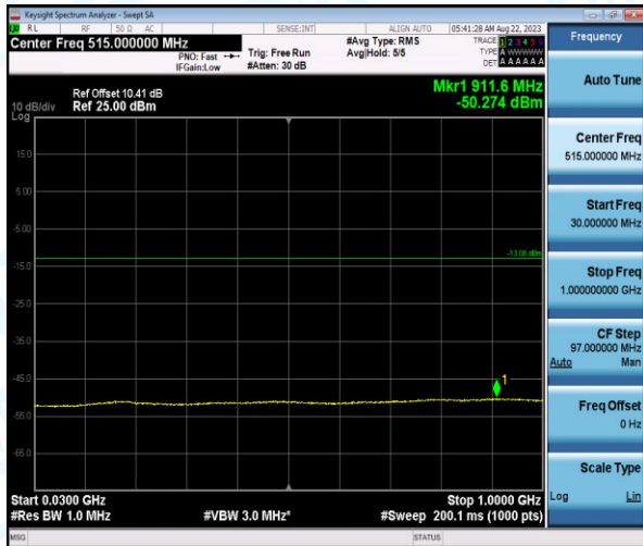
Band4-1.4MHz-QPSK-20175-1-0-Low-30-1000--50.27-PASS
