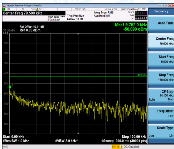
Band4-5MHz-16QAM-20175-1-0-Low-0.009-0.15--56.09-PASS
