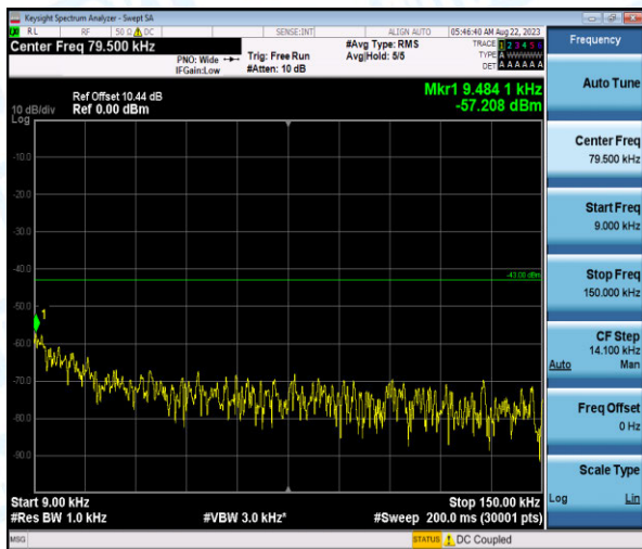
Band4-1.4MHz-16QAM-20393-1-0-High-0.009-0.15--57.21-PASS
