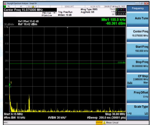
Band4-15MHz-16QAM-20025-1-0-Low-0.15-30--60.36-PASS
