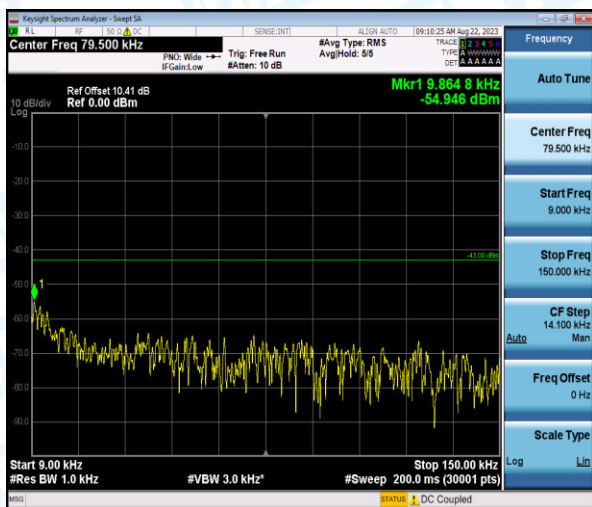
Band4-15MHz-16QAM-20175-1-0-Low-0.009-0.15--54.95-PASS
