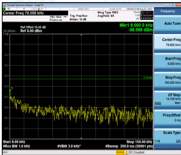
Band4-10MHz-QPSK-20350-1-0-High-0.009-0.15--56.6-PASS
