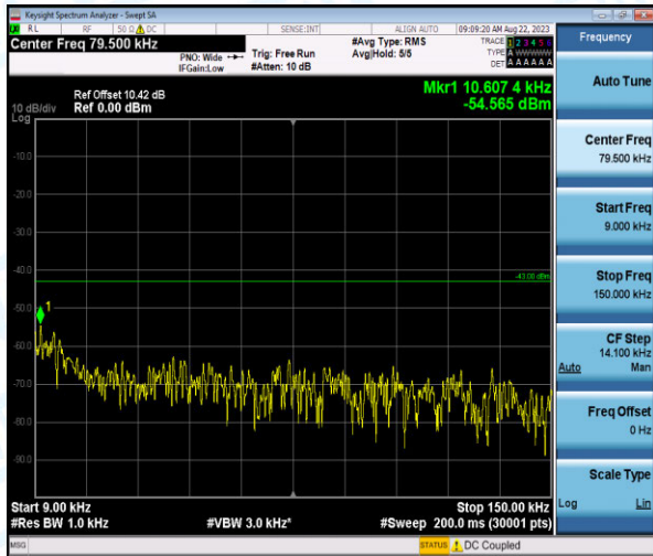
Band4-15MHz-16QAM-20025-1-0-Low-0.009-0.15--54.57-PASS
