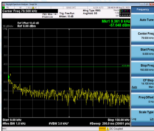
Band4-10MHz-16QAM-20350-1-0-High-0.009-0.15--57.05-PASS
