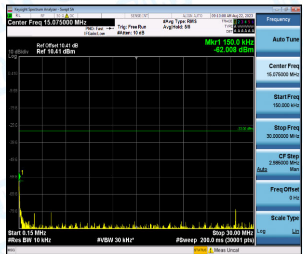
Band4-15MHz-QPSK-20025-1-0-Low-0.15-30--62.01-PASS
