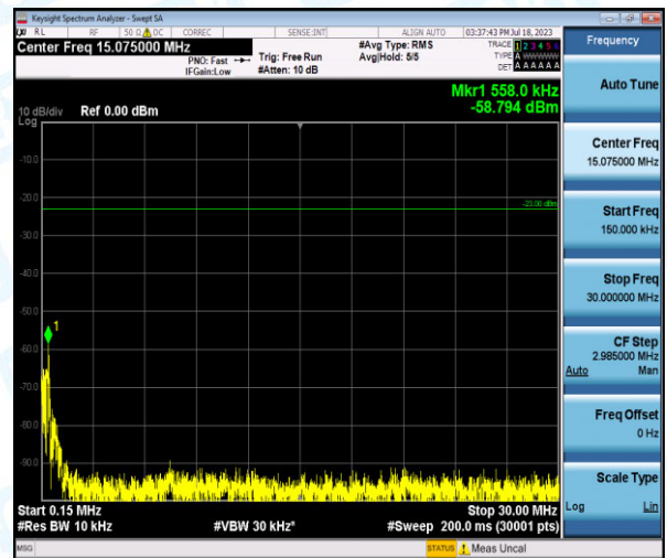
Band5-1.4MHz-QPSK-20643-1-0-High-0.15-30--58.79-PASS
