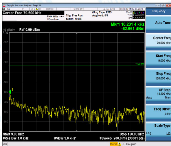
Band5-1.4MHz-16QAM-20643-1-0-High-0.009-0.15--62.66-PASS
