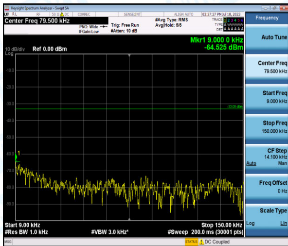
Band5-1.4MHz-QPSK-20643-1-0-High-0.009-0.15--64.53-PASS
