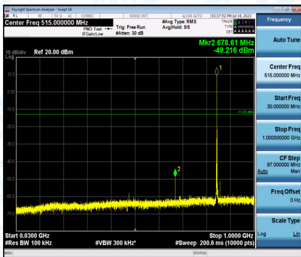
Band5-1.4MHz-QPSK-20643-1-0-High-30-1000--49.22-PASS
