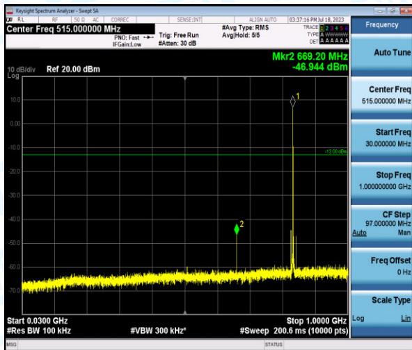
Band5-1.4MHz-16QAM-20525-1-0-Low-30-1000--46.94-PASS
