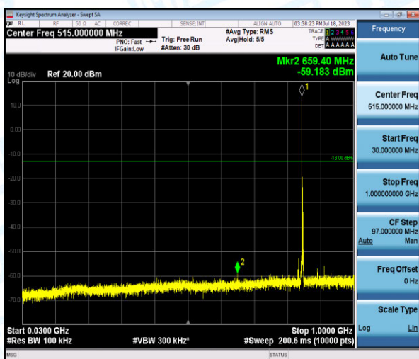
Band5-1.4MHz-16QAM-20643-1-0-High-30-1000--59.18-PASS
