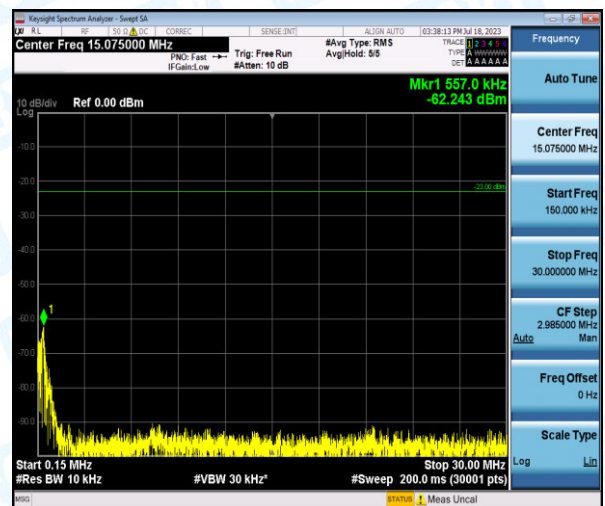
Band5-1.4MHz-16QAM-20643-1-0-High-0.15-30--62.24-PASS
