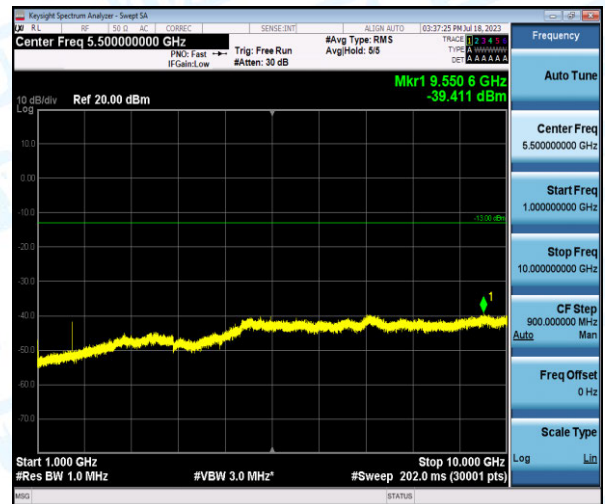
Band5-1.4MHz-16QAM-20525-1-0-Low-1000-10000--39.41-PASS
