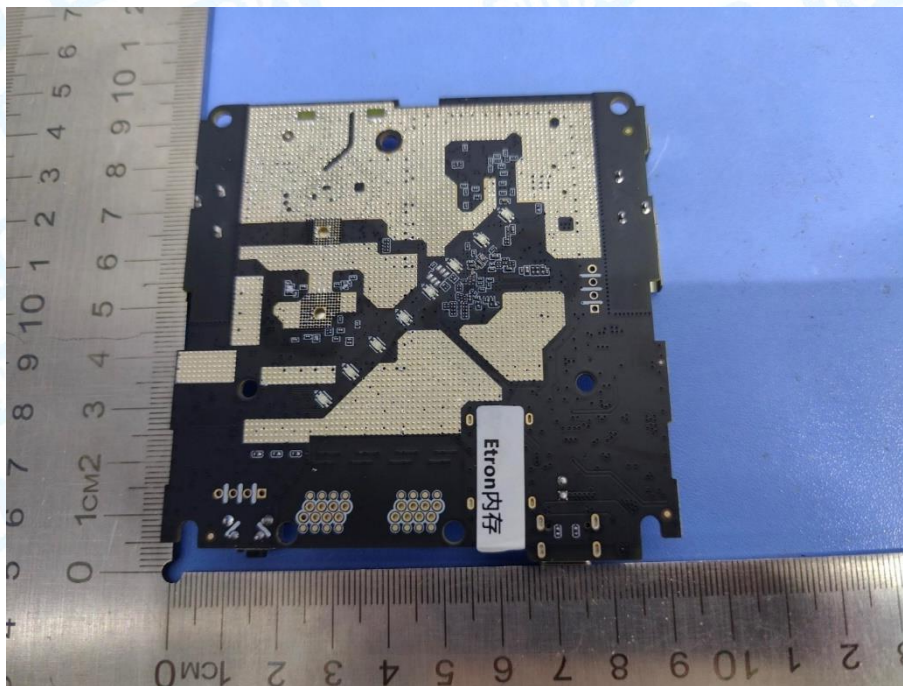
Photo 12 Appearance of PCB(GD)
