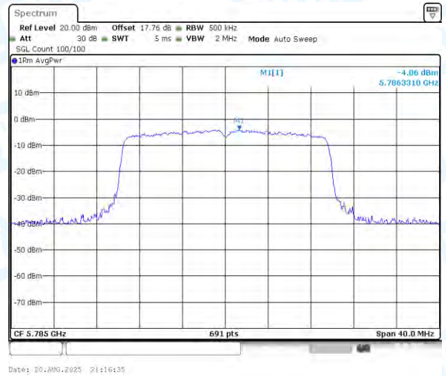
11AX20MIMO-Ant2-5785-PASS
