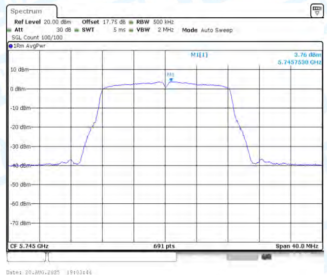
11A-Ant2-5745-PASS
