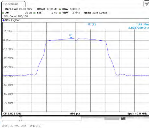
11A-Ant2-5825-PASS
