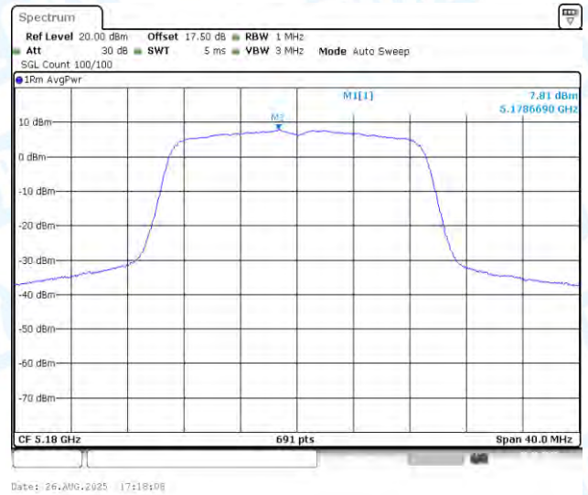
11AC20MIMO-Ant2-5180-PASS
