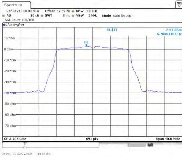
11A-Ant1-5785-PASS
