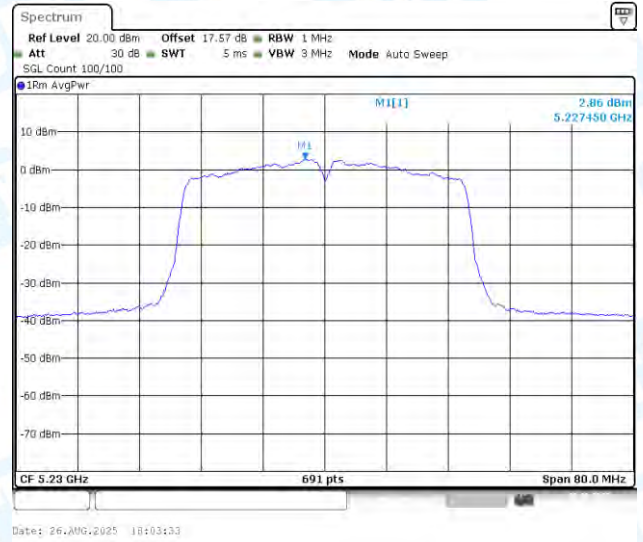
11AC40MIMO-Ant2-5230-PASS
