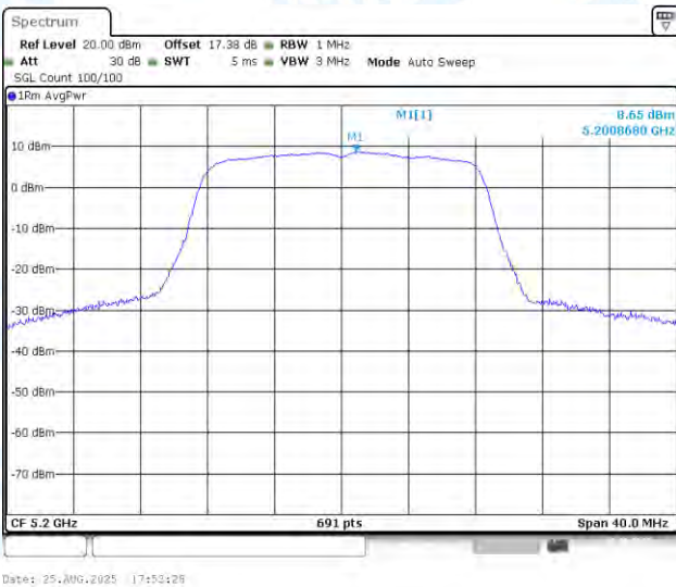
11A-Ant1-5200-PASS
