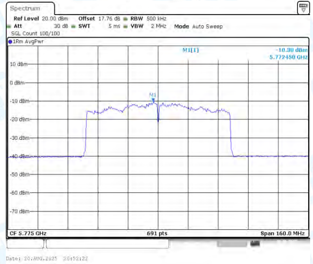
11AC80MIMO-Ant2-5775-PASS
