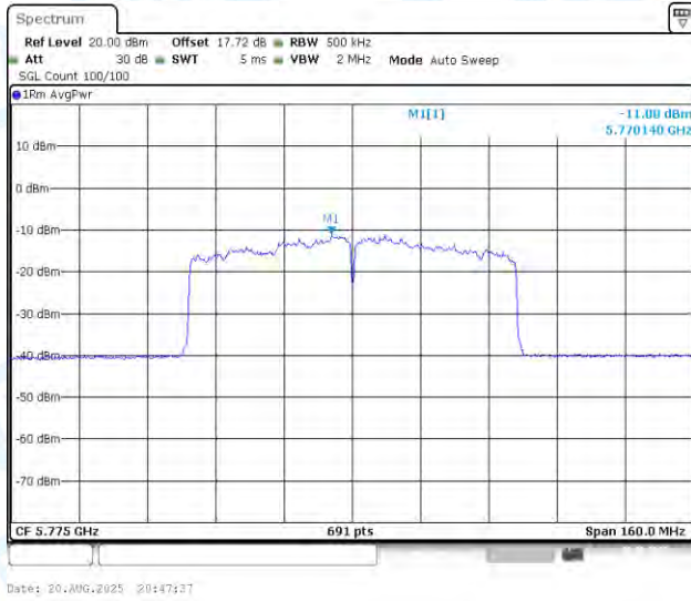
11AC80MIMO-Ant1-5775-PASS
