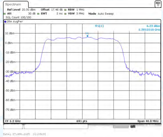
11AX20MIMO-Ant2-5200-PASS
