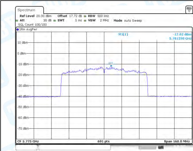
11AX80MIMO-Ant1-5775-PASS
