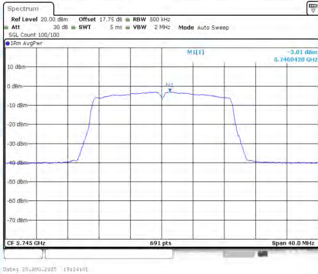
11N20MIMO-Ant1-5745-PASS
