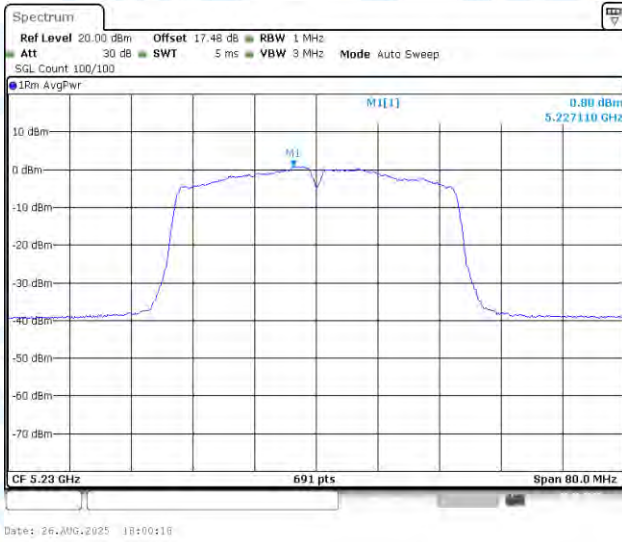
11AC40MIMO-Ant1-5230-PASS
