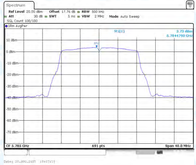
11A-Ant2-5785-PASS
