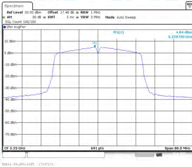
11N40MIMO-Ant1-5230-PASS
