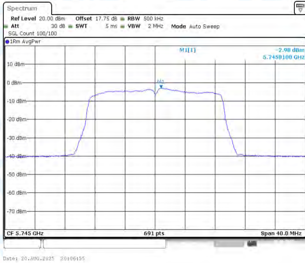
11AC20MIMO-Ant1-5745-PASS
