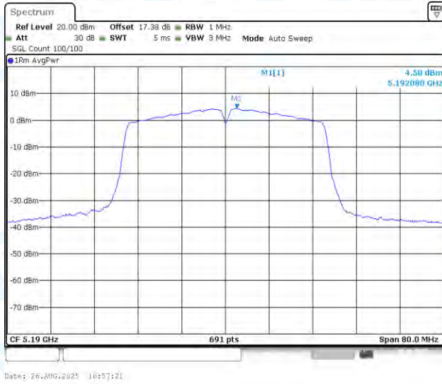
11N40MIMO-Ant1-5190-PASS
