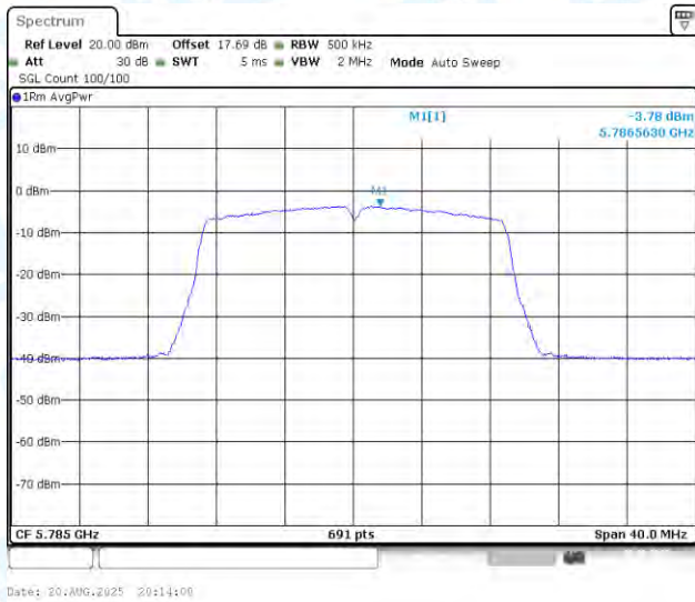
11AC20MIMO-Ant1-5785-PASS
