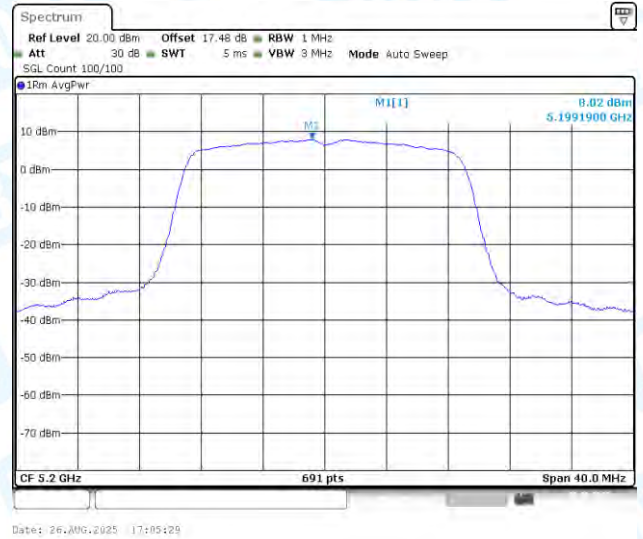
11N20MIMO-Ant2-5200-PASS
