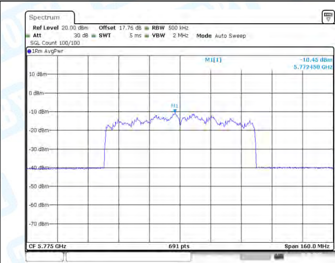
11AX80MIMO-Ant2-5775-PASS
