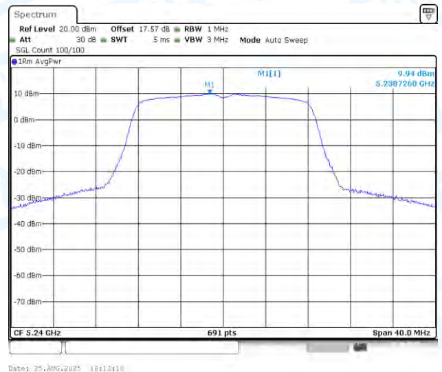
11A-Ant2-5240-PASS
