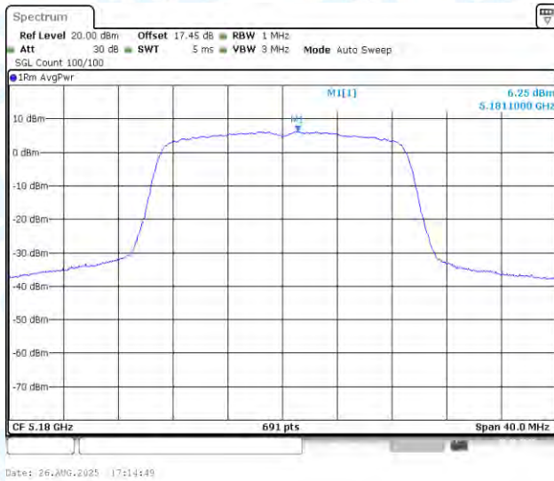
11AC20MIMO-Ant1-5180-PASS
