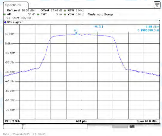
11A-Ant2-5200-PASS
