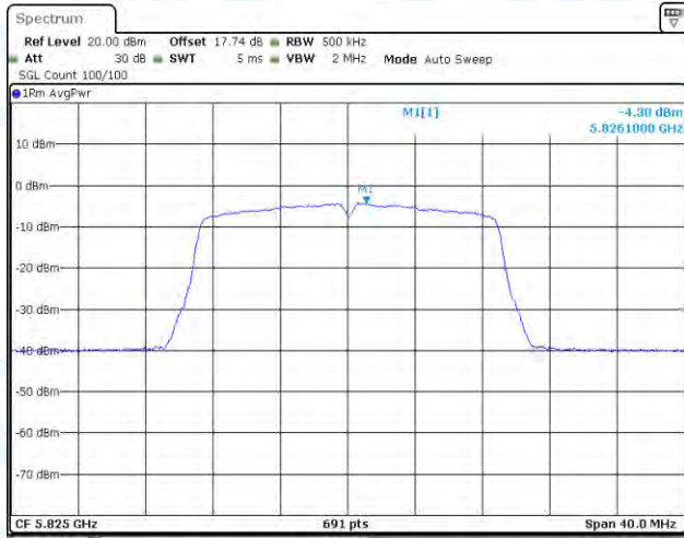
11AC20MIMO-Ant1-5825-PASS
