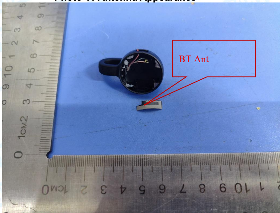
Photo 11 Antenna Appearance
