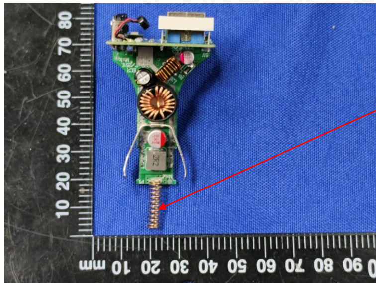
FM Antenna
