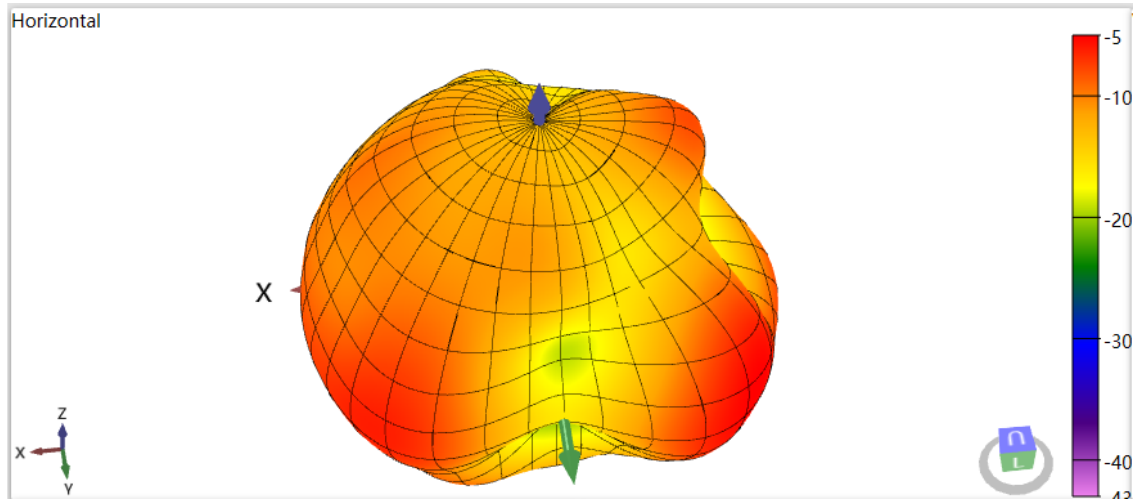
ANT 2440MHz 3D-Horizontal Pattern
