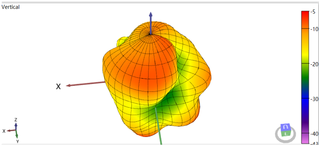
ANT 2440MHz 3D-Vertical Pattern
