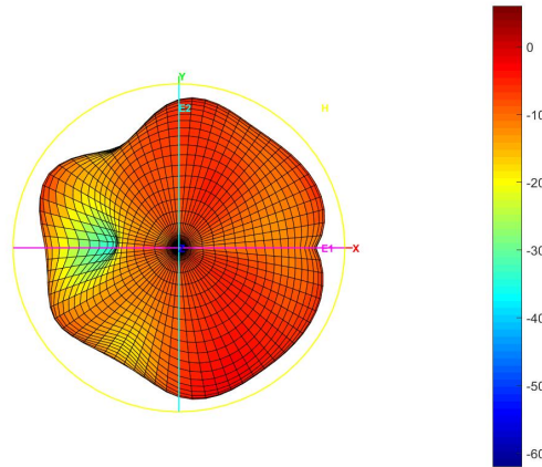
Phi_3D_H_2.45GHz
