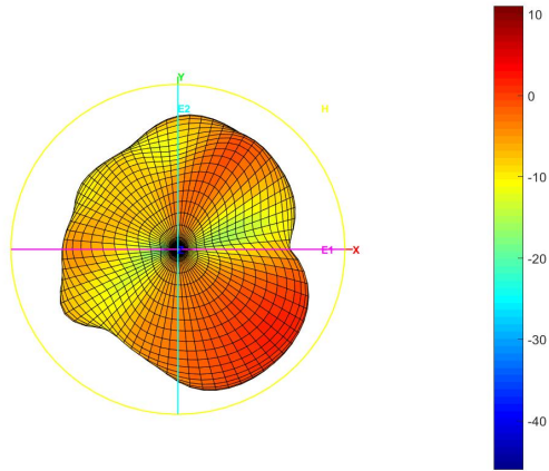
Phi_3D_H_5.5GHz
