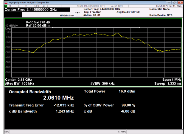
RF PHY 2Mbps 2440MHz
