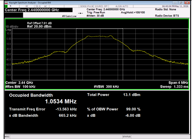
RF PHY 1Mbps 2440MHz
