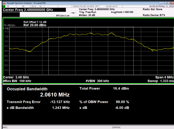
RF PHY 2Mbps 2480MHz
