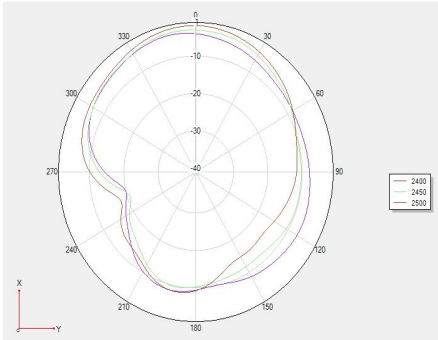
Theta 90 2D
