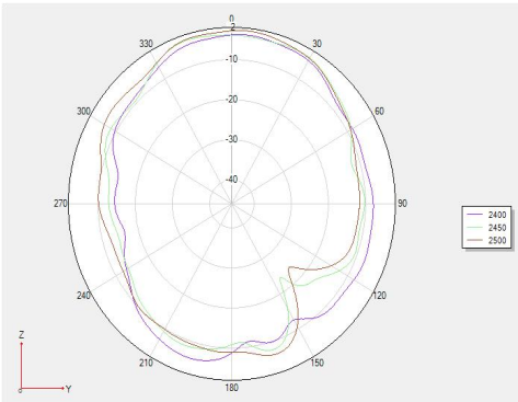
Phi 90 2D
