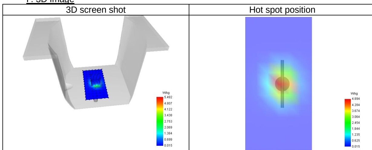
Appendix C. Plots of High SAR Measurement
