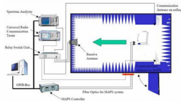
(Testing by 3D anechoic chamber)
