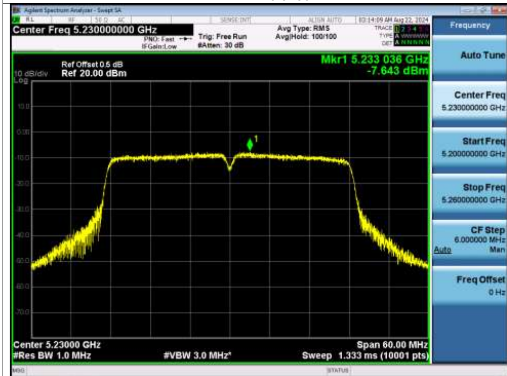
PSD NVNT n40 5230MHz
