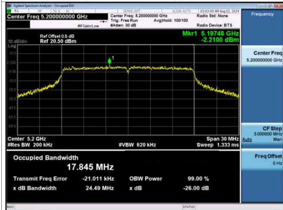
-26dB Bandwidth NVNT ac20 5200MHz
