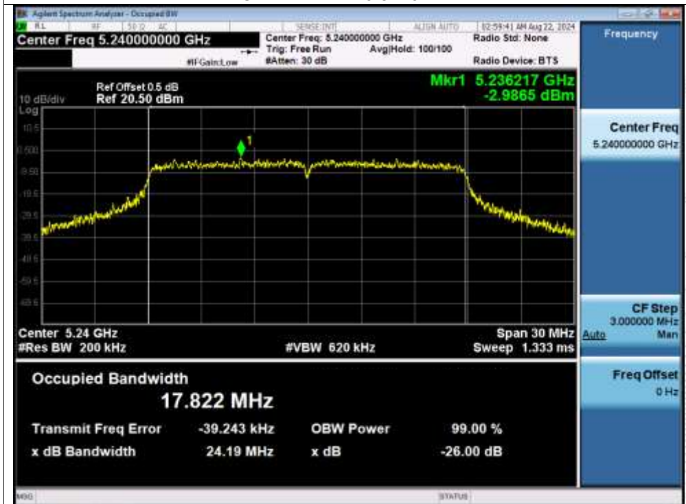
OBW NVNT n20 5240MHz
