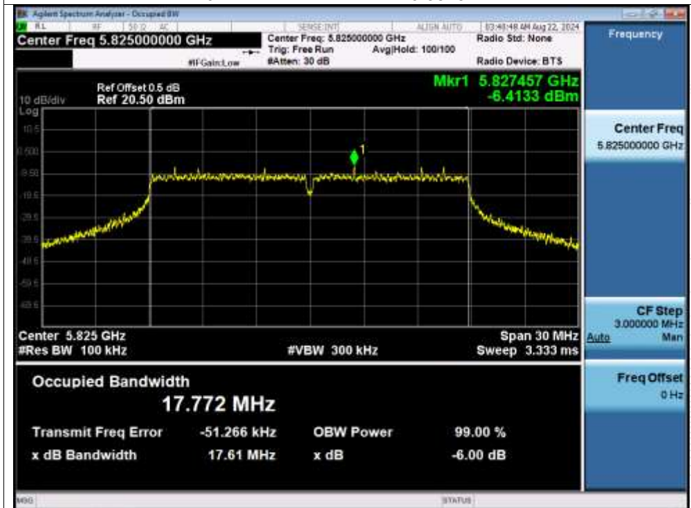
-6dB Bandwidth NVNT n20 5825MHz
