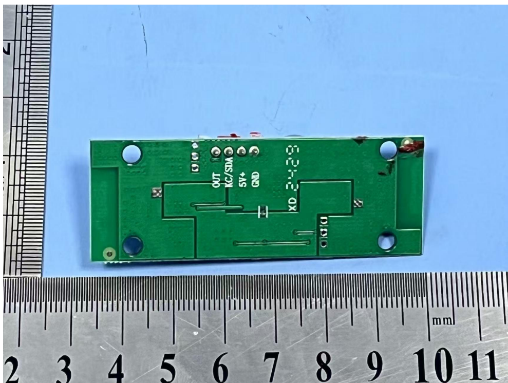
Internal Photos
