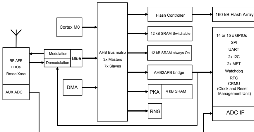
Figure 1. BlueNRG-1 architecture
