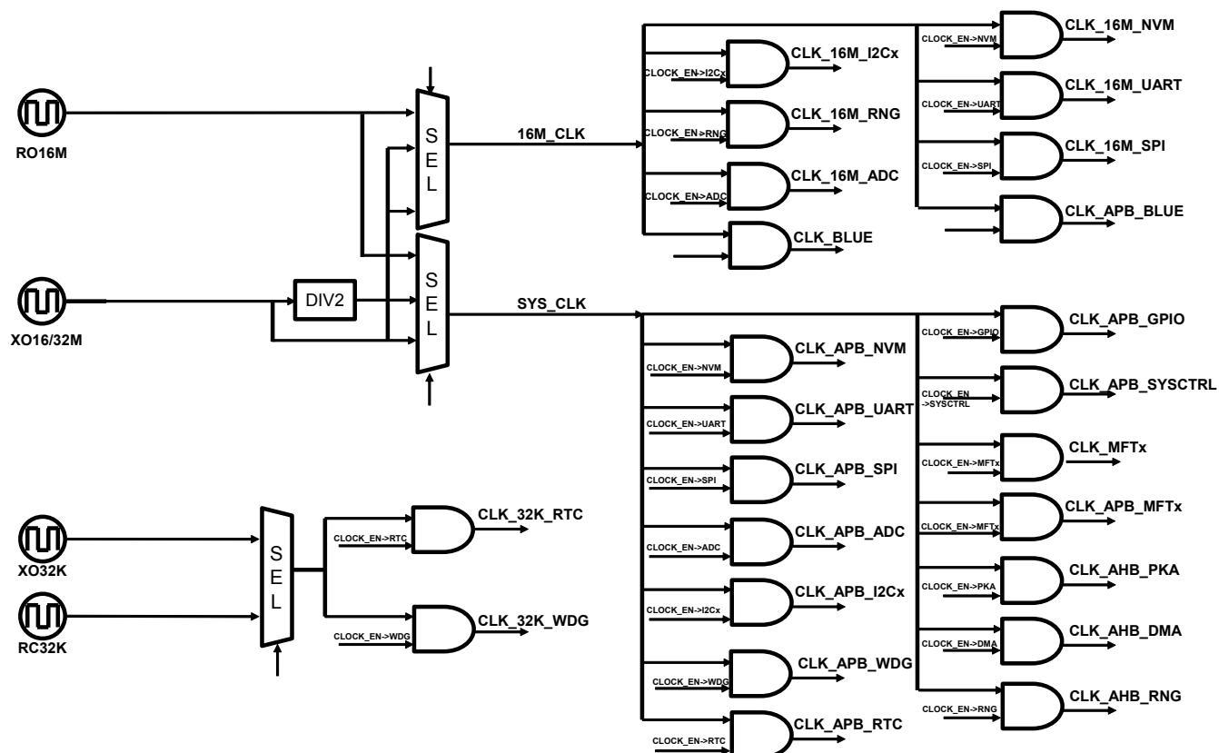
Figure 6. Clock tree
