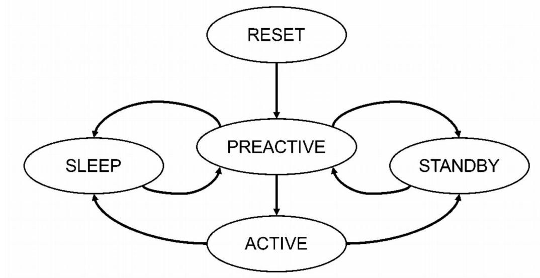
Figure 5. BlueNRG-1 power management state machine
