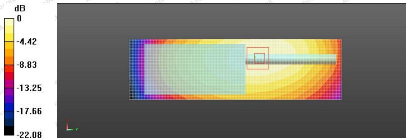
Figure 2: PMR_FM12.5KHz_Body Worn_0mm
