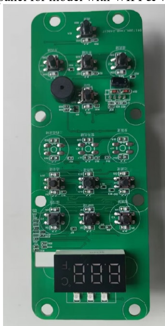
Description: Control panel for model with WIFI & without Ozone function
