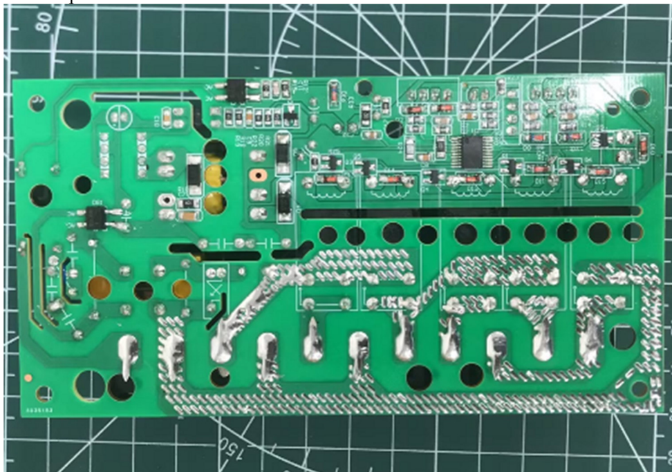
Description: Power PCB view for model with Wifi function & without Ozone function
