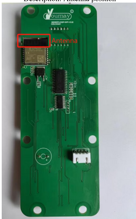
Description: Antenna position
