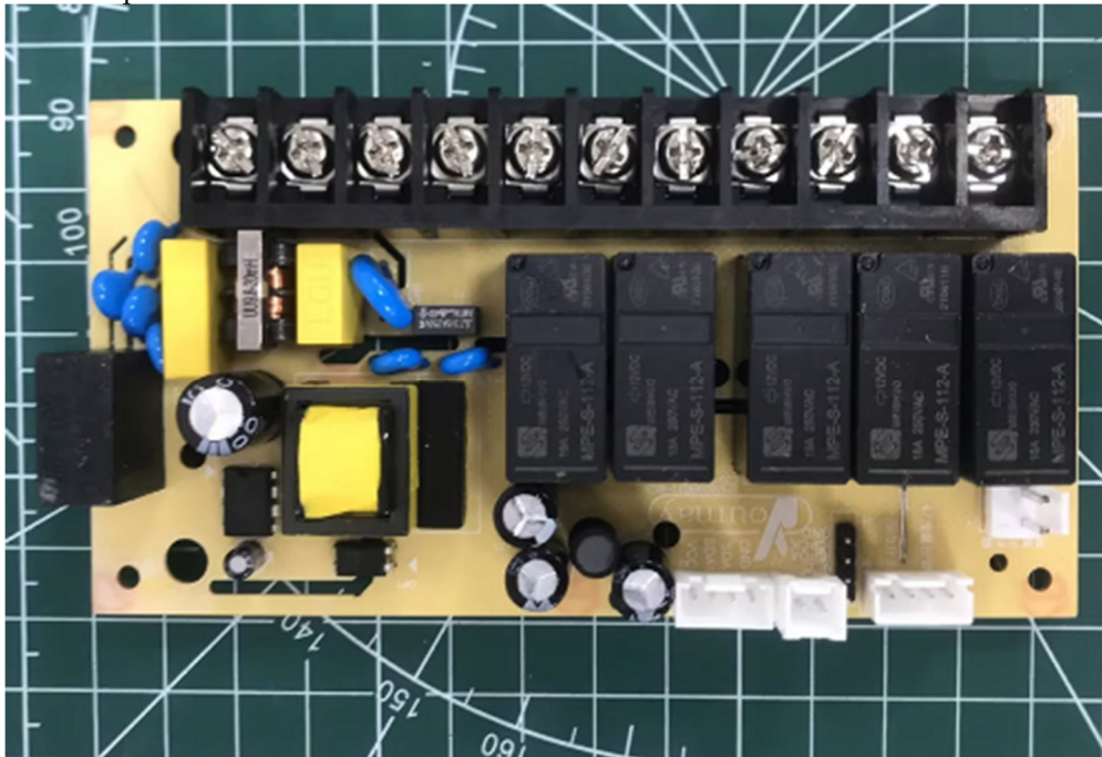
Description: Power PCB view for model with Wifi function & without Ozone function
