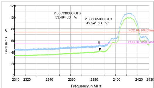
802.11b-Channel 1 Peak+ Average
