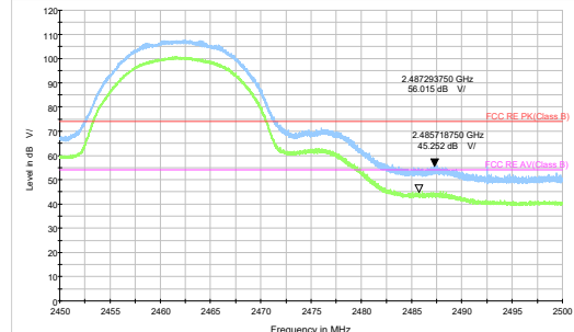
802.11b-Channel 11 Peak+ Average
