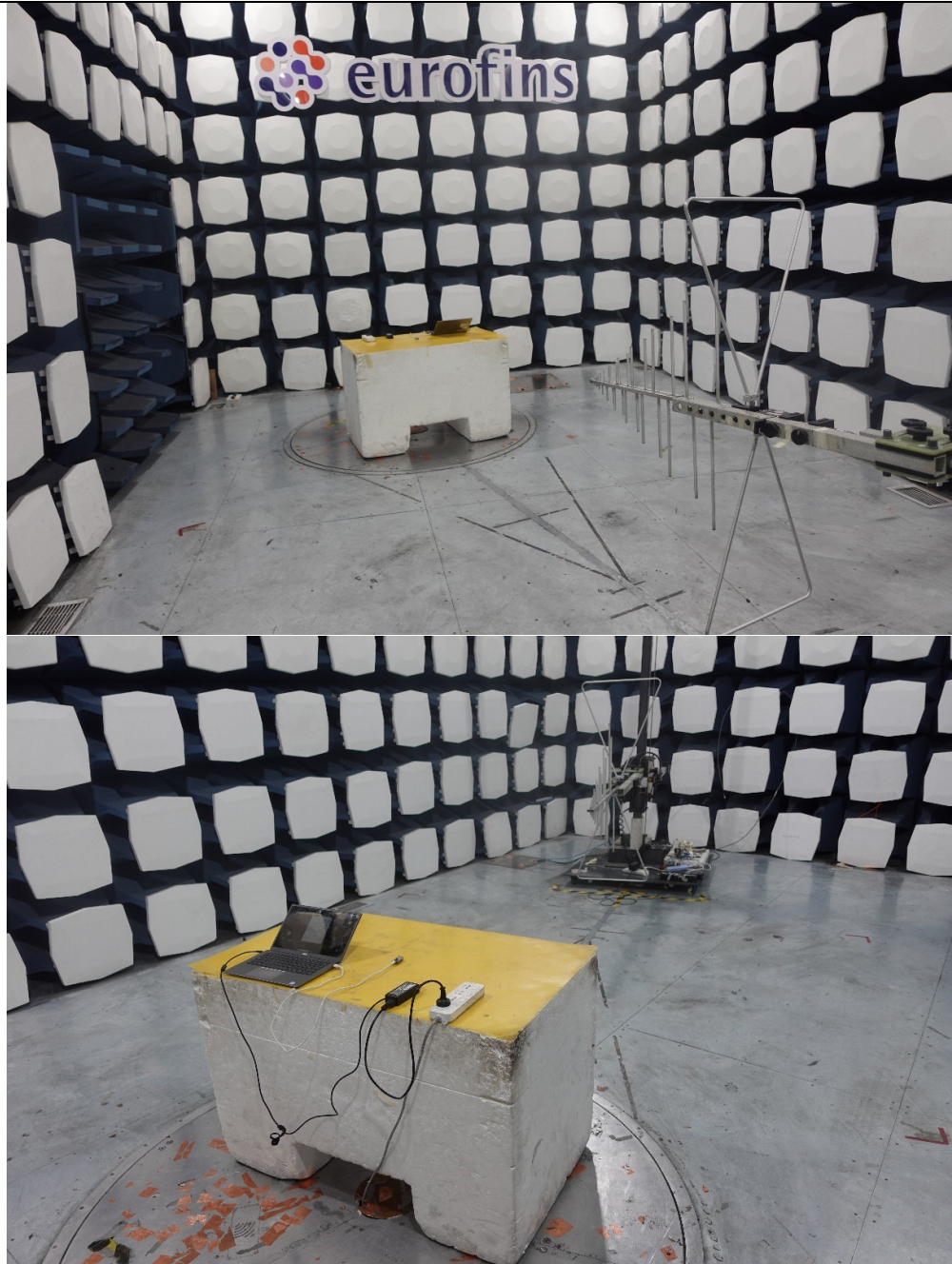
30MHz-1GHz
