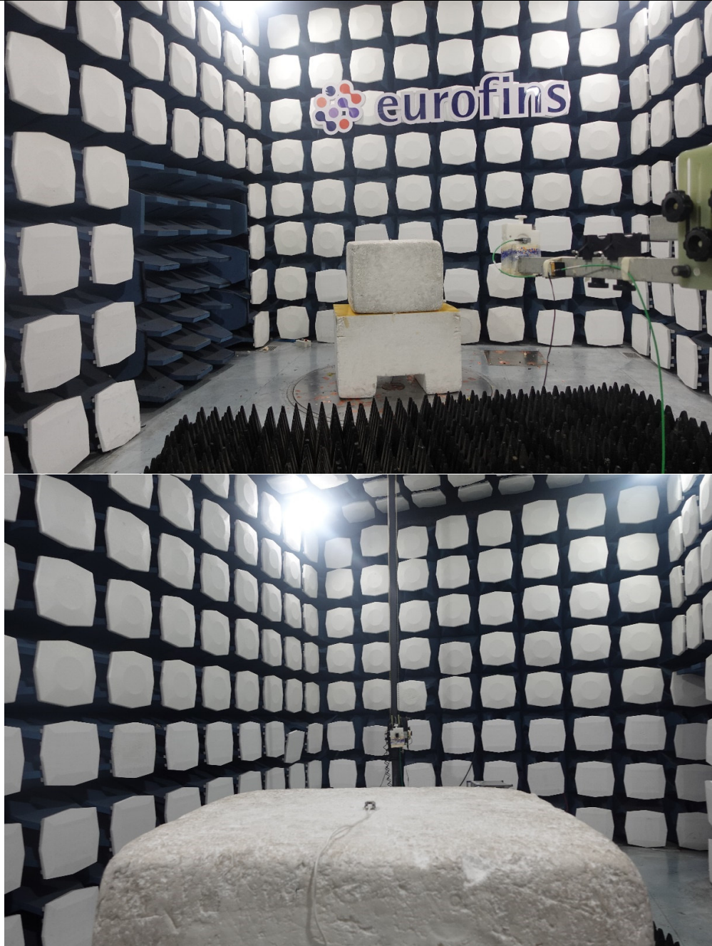
Picture 1 Radiated Emission Test Setup
