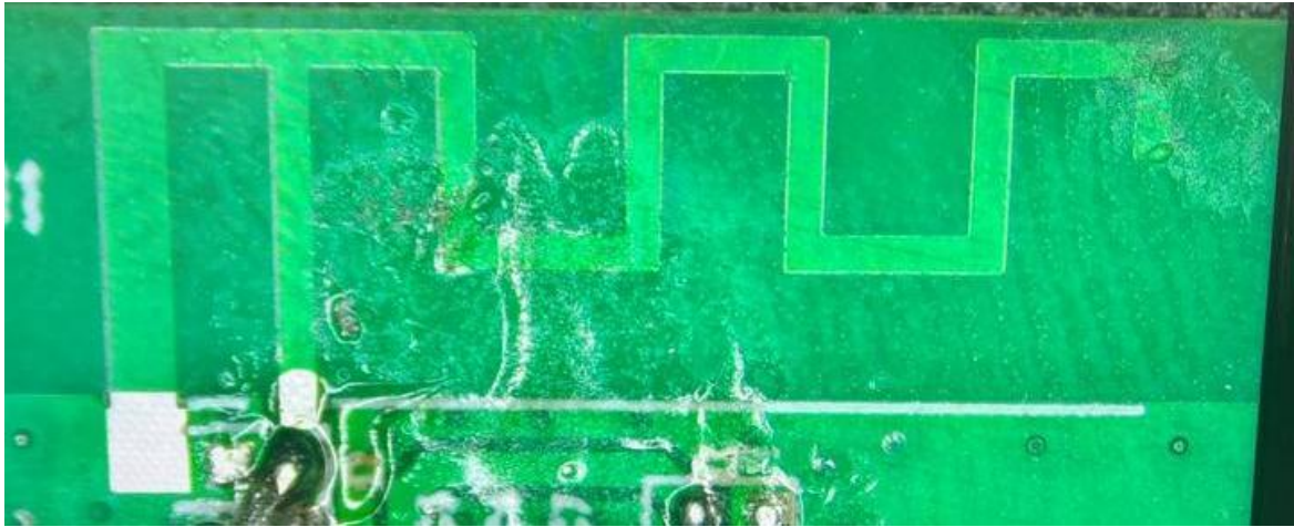
The actual antenna and its physical dimensions
