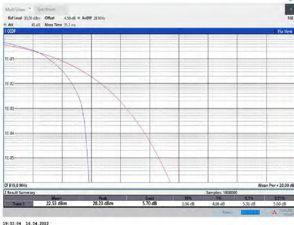
Band26-10MHz-16QAM-26740-50RB#0
