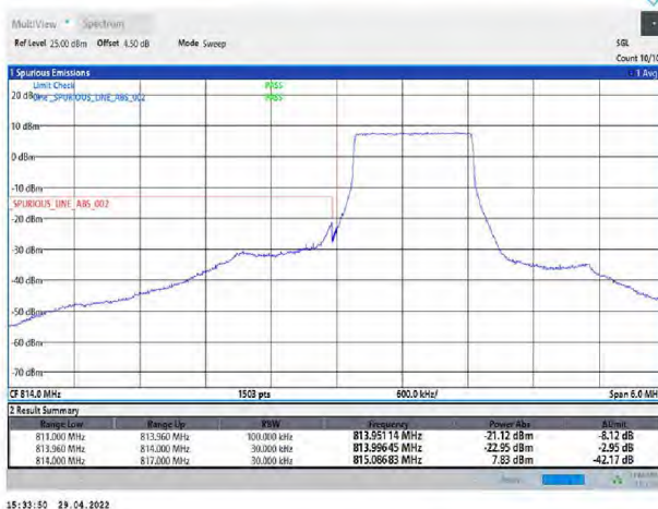
Band26-1.4MHz-QPSK-26697-6RB#0
