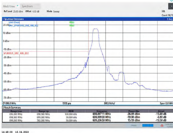
Band12-1.4MHz-QPSK-23017-6RB#0
