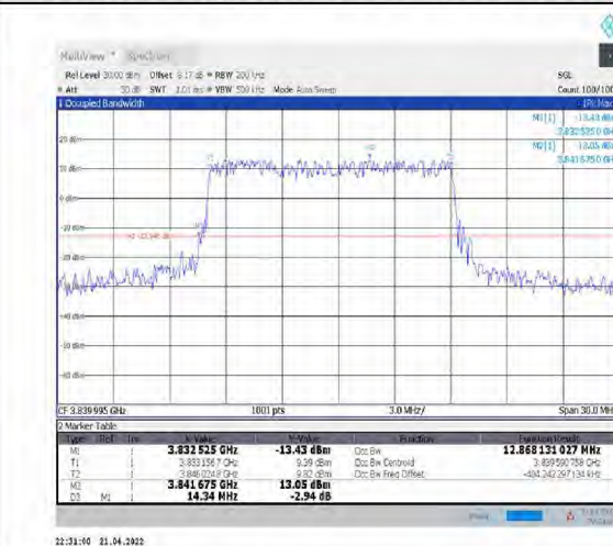
1-N77-3700-3980--30-15-M-4-DFT-64QAM-Outer_Full-36@0-Ant1-12.868-14.340-≤15-PASS
