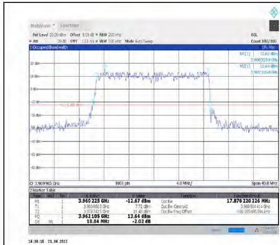
1-N77-3700-3980--30-20-H-1-DFT-QPSK-Outer_Full-50@0-Ant1-17.876-18.840-<20-PASS
