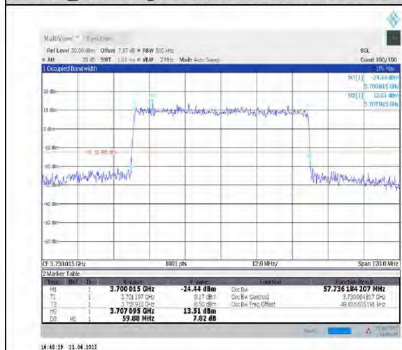
1-N77-3700-3980--30-60-L-1-DFT-QPSK-Outer_Full-162@0-Ant1-57.736-59.880-<60-PASS
