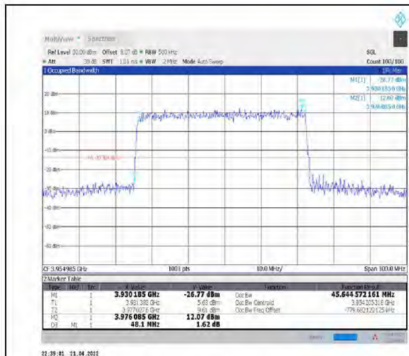
1-N77-3700-3980--30-50-H-4-DFT-64QAM-Outer_Full-128@0-Ant1-45.645-48.100≤50-PASS
