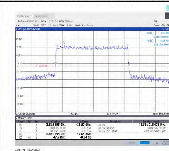
1-N77-3700-3980--30-50-M-4-DFT-64QAM-Outer_Full-128@0-Ant1-45.591-47.500-≤50-PASS
