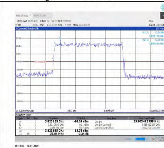
1-N77-3700-3980--30-40-M-1-DFT-QPSK-Outer_Full-100@0-Ant1-35.718-37.840-≤40-PASS
