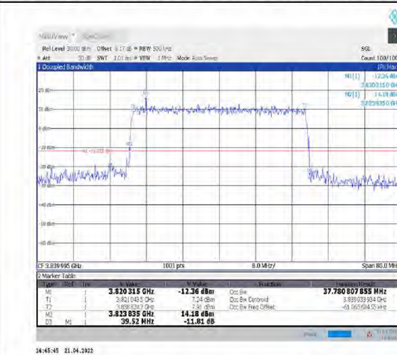
1-N77-3700-3980--30-40-M-7-CP-16QAM-Outer_Full-106@0-Ant1-37.803-39.520-≤40-PASS
