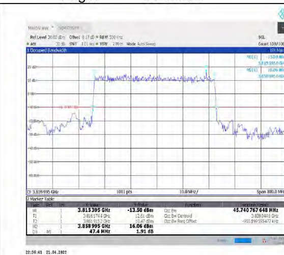
1-N77-3700-3980--30-50-M-2-DFT-PI2BPSK-Outer_Full-128@0-Ant1-45.741-47.400-≤50-PASS
