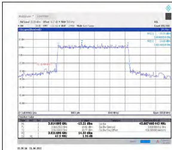
1-N77-3700-3980--30-50-M-1-DFT-QPSK-Outer_Full-128@0-Ant1-45.668-47.900-≤50-PASS
