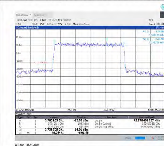
1-N77-3700-3980--30-50-L-1-DFT-QPSK-Outer_Full-128@0-Ant1-45.778-48.000-<50-PASS
