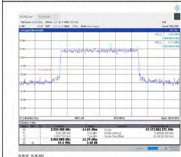
1-N77-3700-3980--30-50-H-6-CP-QPSK-Outer_Full-133@0-Ant1-47.473-49.000≤50-PASS
