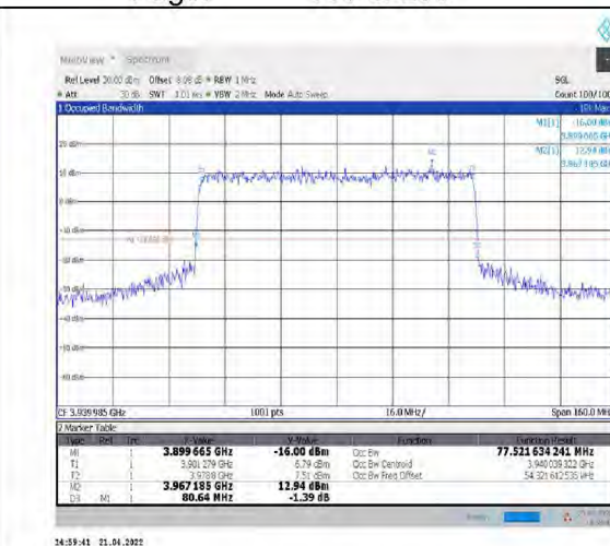
1-N77-3700-3980--30-80-H-8-CP-64QAM-Outer_Full-217@0-Ant1-77.522-80.640-<80-PASS
