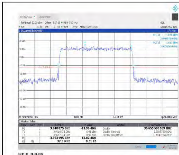
1-N77-3700-3980--30-40-H-3-DFT-16QAM-Outer_Full-100@0-Ant1-35.662-37.600-≤40-PASS
