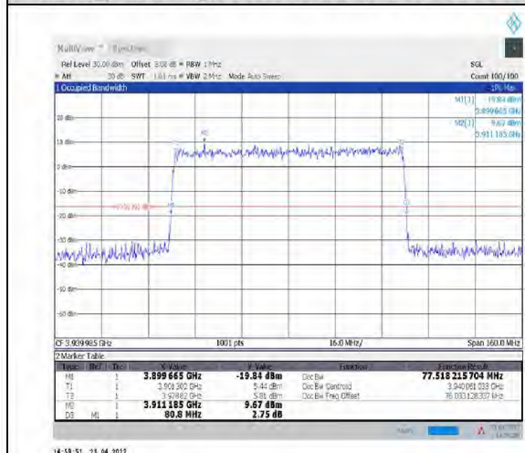
1-N77-3700-3980--30-80-H-9-CP-256QAM-Outer_Full-217@0-Ant1-77.518-80.800-<80-PASS
