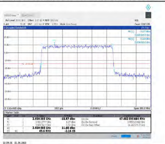
1-N77-3700-3980--30-50-H-7-CP-16QAM-Outer_Full-133@0-Ant1-47.484-49.600≤50-PASS
