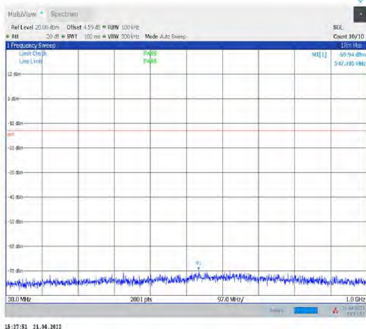
1-N77-3700-3980--30-100-H-1-DFT-PI2BPSK- Inner_1RB_Left-1@1-30-1000-Ant1--69.94--13- PASS
