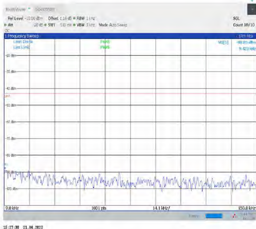
1-N77-3700-3980--30-100-H-1-DFT-PI2BPSK- Inner_1RB_Left-1@1-0.009-0.15-Ant1--88.80--43- PASS
