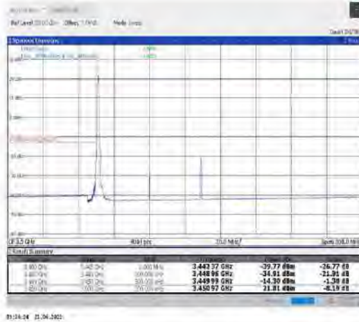
1-N78-3450-3550--30-60-L-1-DFT-PI2BPSK-Edge_1RB_Left-1@0-Ant1-PASS-see graph
