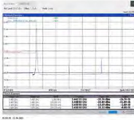
1-N78-3450-3550--30-100-L-1-DFT-PI2BPSK-Edge_1RB_Left-1@0-Ant1-PASS-see graph
