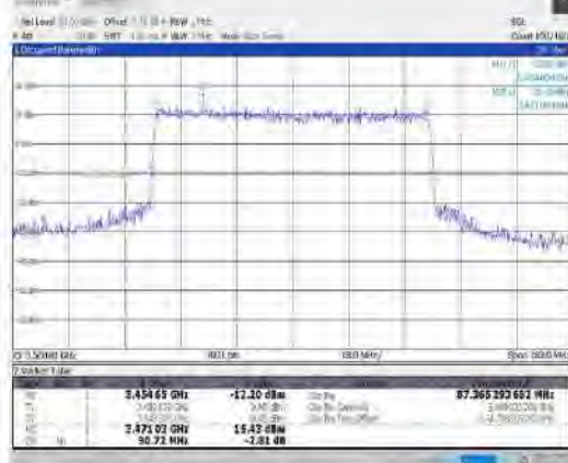
1-N78-3450-3550--30-90-M-6-CP-QPSK-Outer_Full- 245@0-Ant1-87.365-90.720-≤90-PASS
