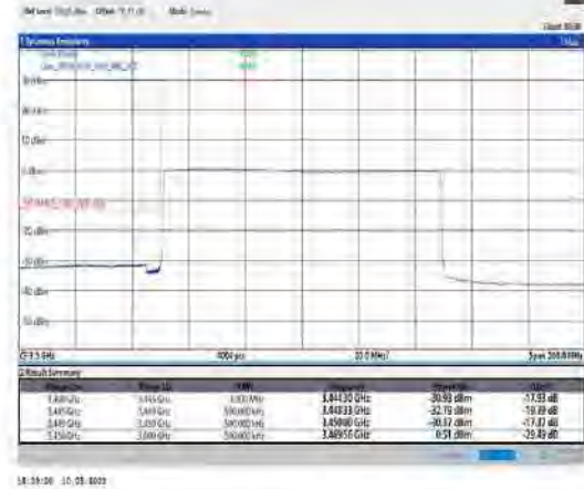
1-N78-3450-3550-PC2-30-100-L-6-CP-QPSK-Outer_Full-273@0-Ant1-PASS-see graph
