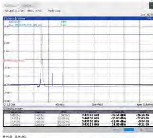
1-N78-3450-3550-30-30-L-4-CP-QPSK-Edge_1RB_Left-1@0-Ant1-PASS-see graph
