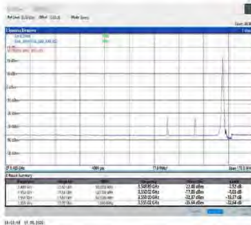
1-N78-3450-3550-PC2-30-40-H-5-CP-QPSK-Edge_1RB_Right-1@105-Ant1-PASS-see graph
