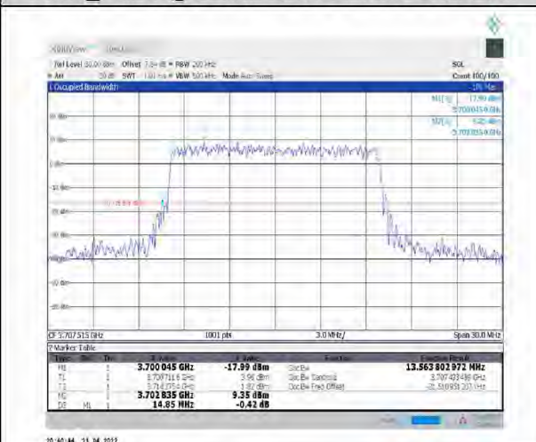
1-N78-3700-3800--30-15-L-9-CP-256QAM- Outer Full-38@0-Ant1-13.564-14.850-≤15-PASS
