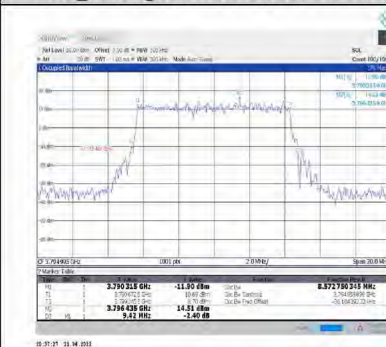
1-N78-3700-3800--30-10-H-2-DFT-PI2BPSK- Outer Full-24@0-Ant1-8.573-9.420≤10-PASS
