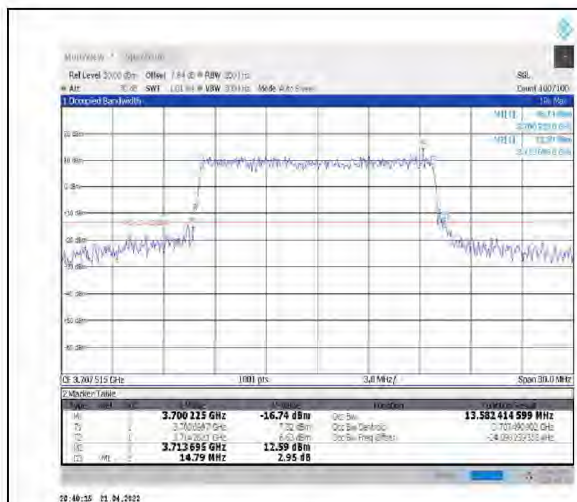
1-N78-3700-3800--30-15-L-6-CP-QPSK-Outer_Full- 38@0-Ant1-13.582-14.790-≤15-PASS
