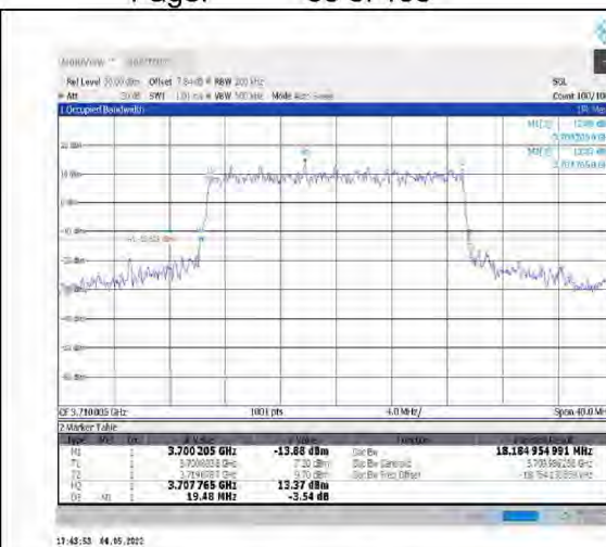
1-N78-3700-3800--30-20-L-8-CP-64QAM- Outer Full-51@0-Ant1-18.185-19.480≤20-PASS
