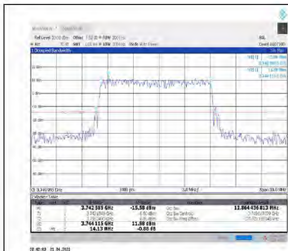
1-N78-3700-3800--30-15-M-5-DFT-256QAM- Outer Full-36@0-Ant1-12.864-14.130-≤15-PASS
