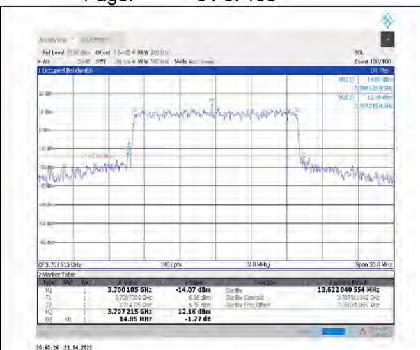
1-N78-3700-3800--30-15-L-7-CP-16QAM- Outer Full-38@0-Ant1-13.622-14.850≤15-PASS
