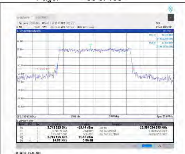
1-N78-3700-3800--30-15-M-6-CP-QPSK-Outer_Full- 38@0-Ant1-13.594-14.880≤15-PASS
