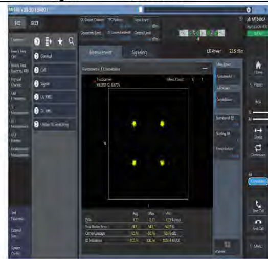
1-N78-3700-3800--30-100-M-6-CP-QPSK-Outer_Full-273@0-Ant1-see graph-PASS
