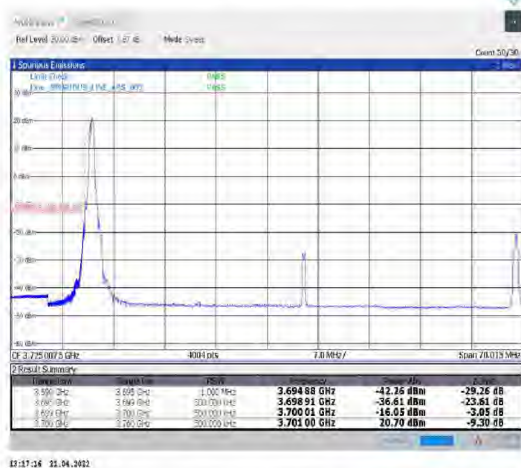
1-N78-3700-3800--30-60-L-4-CP-QPSK- Edge_1RB_Left-1@0-Ant1-PASS-see graph
