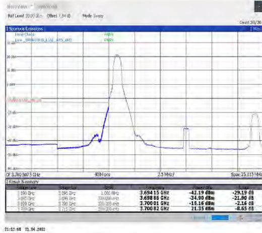
1-N78-3700-3800--30-15-L-1-DFT-PI2BPSK- Edge_1RB_Left-1@0-Ant1-PASS-see graph
