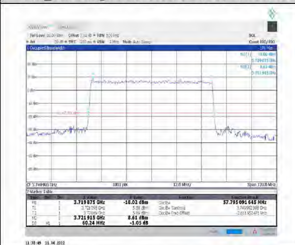
1-N78-3700-3800--30-60-M-9-CP-256QAM- Outer Full-162@0-Ant1-57.795-60.240-<60-PASS
