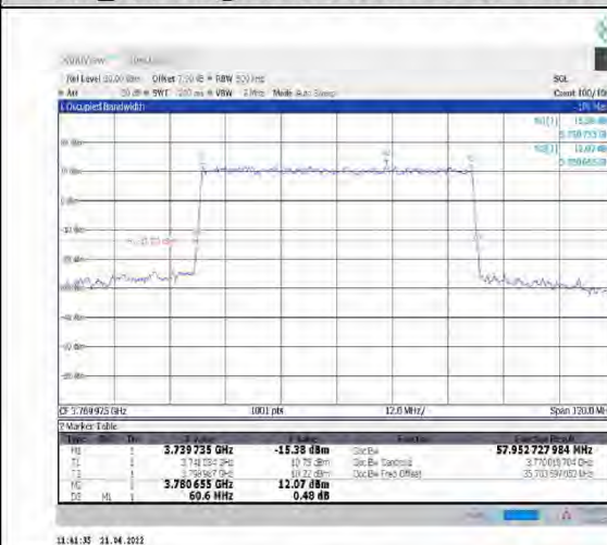
1-N78-3700-3800--30-60-H-4-DFT-64QAM- Outer Full-162@0-Ant1-57.953-60.600-<60-PASS
