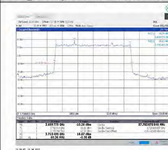
1-N78-3700-3800--30-60-L-2-DFT-PI2BPSK- Outer Full-162@0-Ant1-57.784-60.360-≤60-PASS
