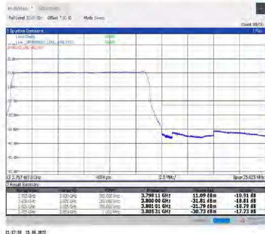
1-N78-3700-3800--30-15-H-3-DFT-PI2BPSK- Outer Full-36@0-Ant1-PASS-see graph
