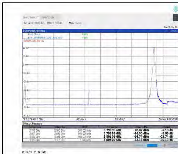
1-N78-3700-3800--30-60-H-2-DFT-PI2BPSK- Edge 1RB Right-1@161-Ant1-PASS-see graph
