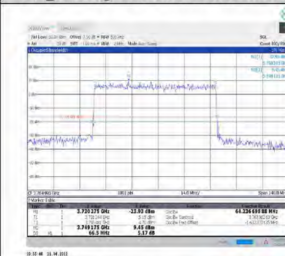
1-N78-3700-3800--30-70-H-5-DFT-256QAM- Outer Full-180@0-Ant1-64.237-66.500≤70-PASS
