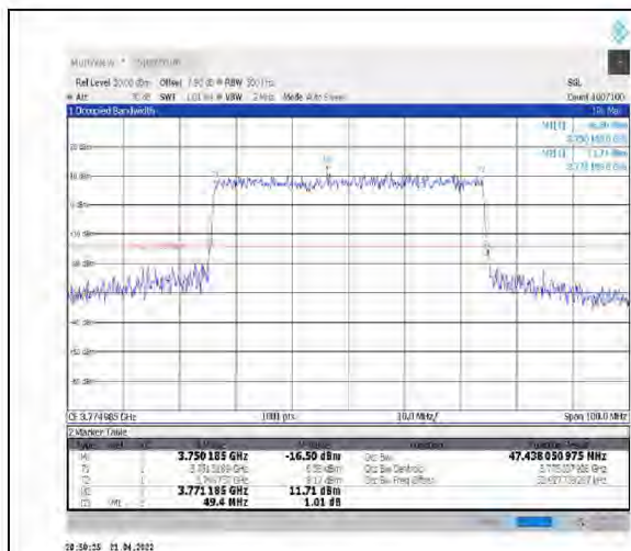
1-N78-3700-3800--30-50-H-8-CP-64QAM- Outer Full-133@0-Ant1-47.438-49.400≤50-PASS
