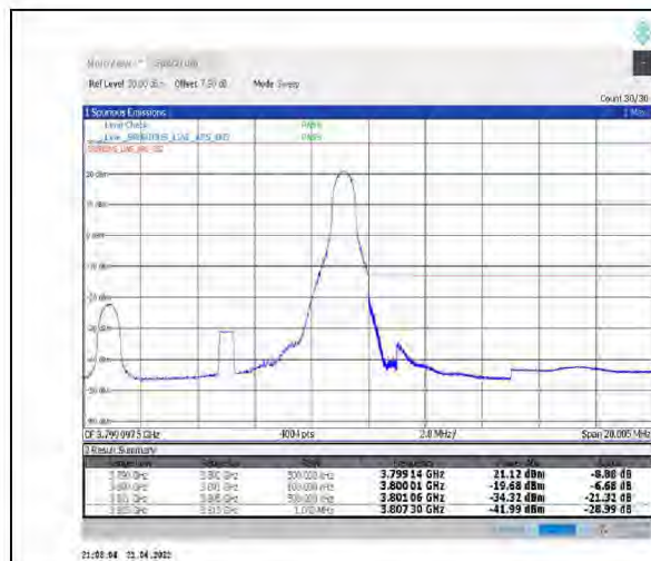
1-N78-3700-3800--30-10-H-2-DFT-PI2BPSK- Edge 1RB Right-1@23-Ant1-PASS-see graph
