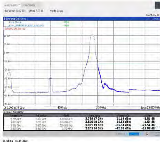
1-N78-3700-3800--30-15-H-2-DFT-PI2BPSK- Edge 1RB Right-1@37-Ant1-PASS-see graph
