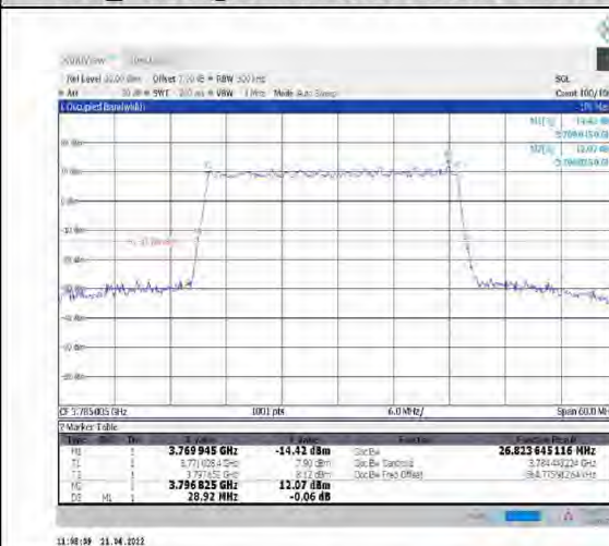
1-N78-3700-3800--30-30-H-5-DFT-256QAM- Outer Full-75@0-Ant1-26.824-28.920-≤30-PASS
