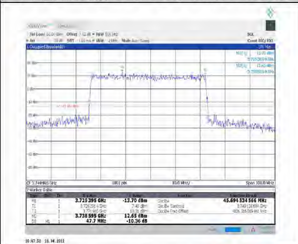
1-N78-3700-3800--30-50-M-4-DFT-64QAM-Outer_Full-128@0-Ant1-45.695-47.700-<50-PASS
