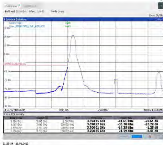
1-N78-3700-3800--30-15-L-4-CP-QPSK- Edge_1RB_Left-1@0-Ant1-PASS-see graph
