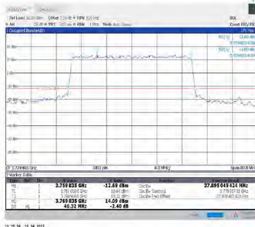
1-N78-3700-3800--30-40-H-6-CP-QPSK-Outer_Full- 106@0-Ant1-37.895-40.320-<40-PASS
