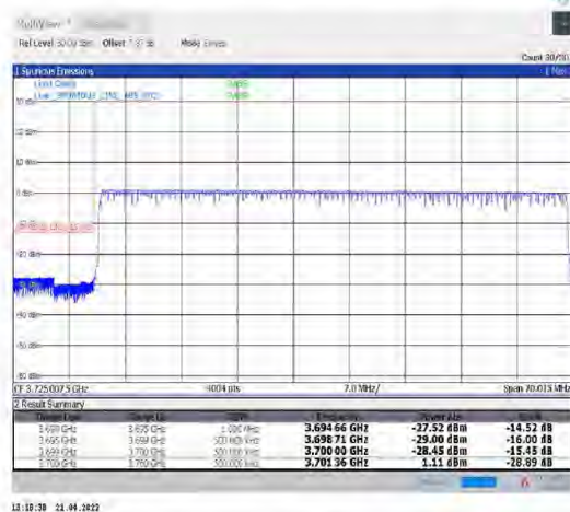
1-N78-3700-3800--30-60-L-6-CP-QPSK- Outer_Full-162@0-Ant1-PASS-see graph
