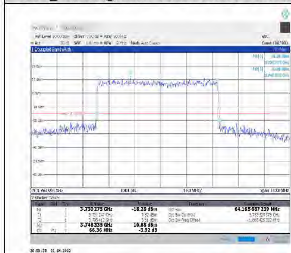
1-N78-3700-3800--30-70-H-4-DFT-64QAM- Outer Full-180@0-Ant1-64.166-66.360-≤70-PASS
