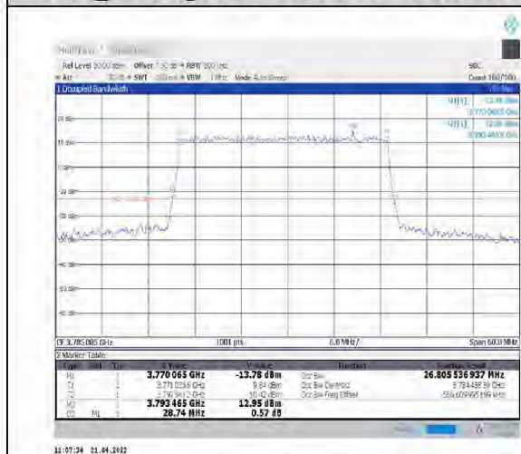
1-N78-3700-3800--30-30-H-4-DFT-64QAM- Outer Full-75@0-Ant1-26.806-28.740-≤30-PASS
