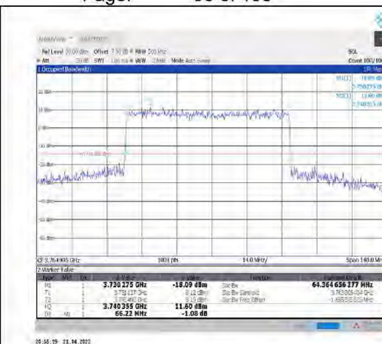
1-N78-3700-3800--30-70-H-3-DFT-16QAM- Outer Full-180@0-Ant1-64.365-66.220-≤70-PASS
