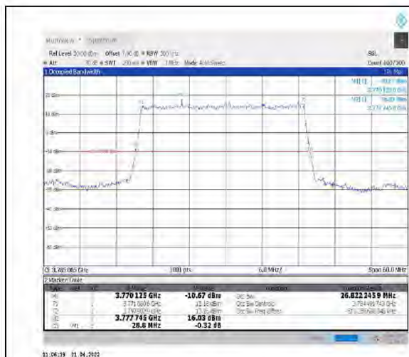
1-N78-3700-3800--30-30-H-2-DFT-PI2BPSK- Outer Full-75@0-Ant1-26.822-28.800-≤30-PASS
