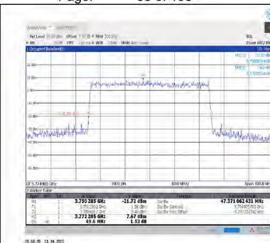
1-N78-3700-3800--30-50-H-9-CP-256QAM- Outer Full-133@0-Ant1-47.371-49.600-≤50-PASS
