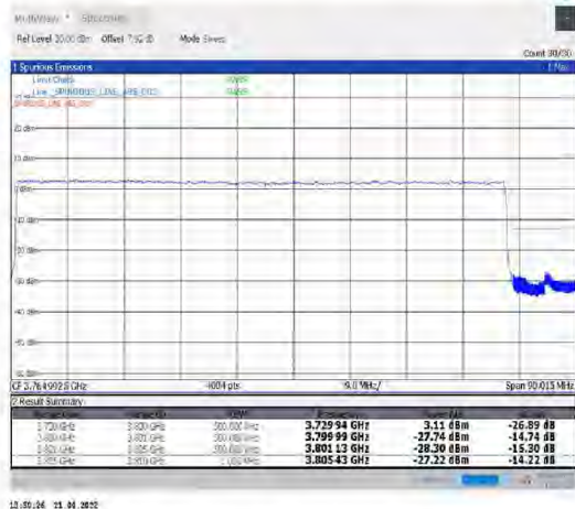
1-N78-3700-3800--30-80-H-3-DFT-PI2BPSK- Outer Full-216@0-Ant1-PASS-see graph
