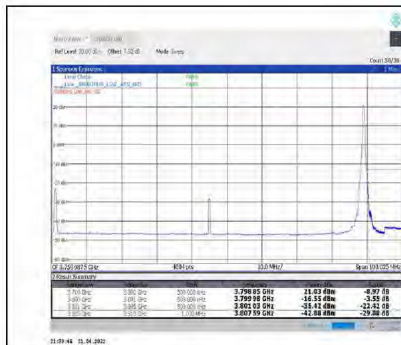
1-N78-3700-3800--30-90-H-2-DFT-PI2BPSK- Edge 1RB Right-1@244-Ant1-PASS-see graph
