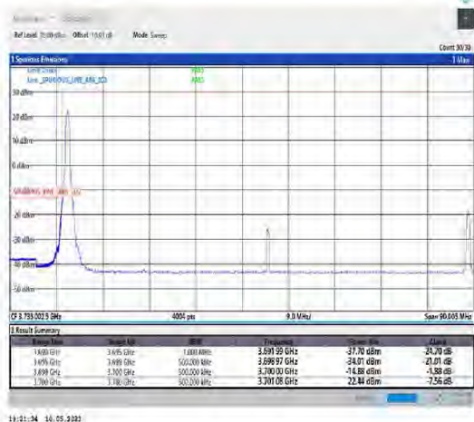
1-N78-3700-3800-PC2-30-80-L-4-CP-QPSK- Edge 1RB Left-1@0-Ant1-PASS-see graph
