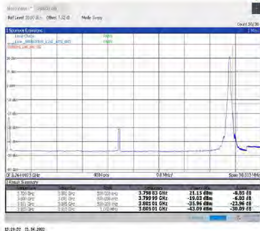
1-N78-3700-3800--30-80-H-2-DFT-PI2BPSK- Edge 1RB Right-1@216-Ant1-PASS-see graph
